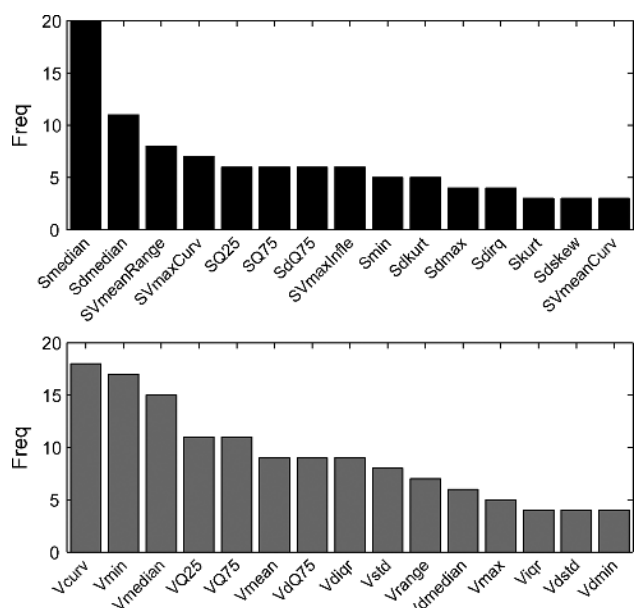
Fig. 6. Most frequently selected features in logistic regression models using forward feature selection. The figures show the sentence-level (top) and voiced-level (bottom) features. The nomenclature of the F0 features is given in Tables II and III.
