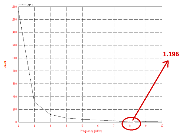
Fig.4.2.5 VSWR vs. frequency graph on RT Duroid
