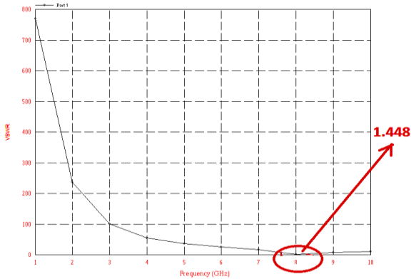
Fig.4.2.3 VSWR vs. frequency graph on RO4003
