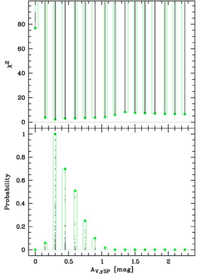
Fig. 7. PDF derivation for A_{V,\text{SP}} . In this example, the discrete model A_{V,\text{SP}} values increase in steps of 0.15 mag. For the description of the plot see Fig. 6.
