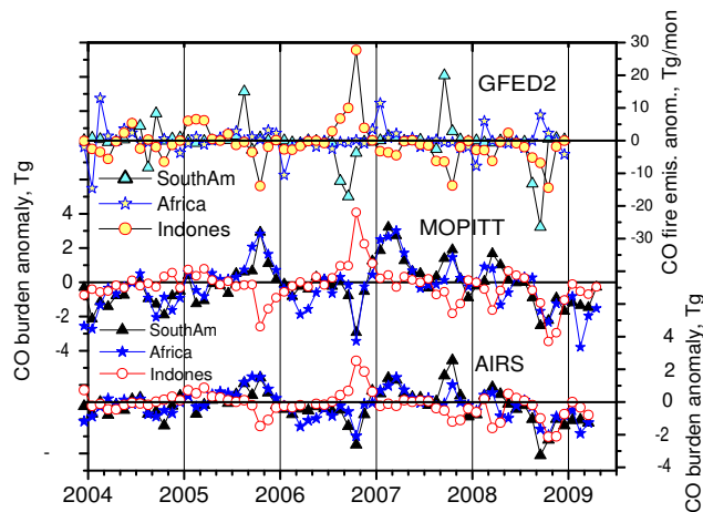
Fig. 13. Anomalies of CO fire emissions according to GFED2 and anomalies of CO burdens measured by MOPITT and AIRS for three regions since 2004.
