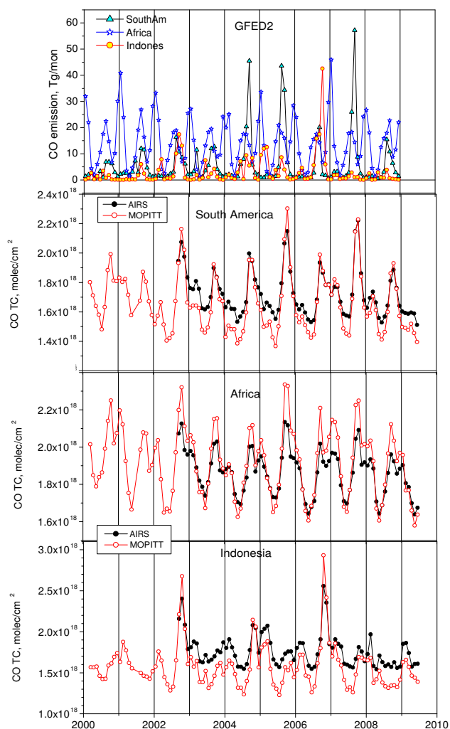
Fig. 12. Corrected monthly mean CO TC from the two satellite sounders averaged over three tropical regions subjected to biomass burning and in comparison with GFED2 emissions.
