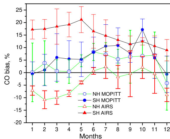
Fig. 3. Seasonal dependence of CO TC bias for two satellite sounders in both hemispheres. Monthly averaged deviations of CO TC measured by satellite sounders from those measured by ground-based spectrometers.
