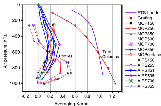
Fig. 1. Examples of averaging kernels for interferometer BRUKER IFS 120HR installed in Lauder, New Zealand (Rinsland et al., 2002), grating spectrometer in Zvenigorod, Russia (Yurganov et al., 2002), MOPITT V3 (Deeter et al., 2004) for 9 September 2000, over the tropical Atlantic, red lines, and AIRS V5 (30 August 2006, 40.1° N, 95.6° W), blue lines. Designation MOP150 means averaging kernel for 150 hPa level, etc.
