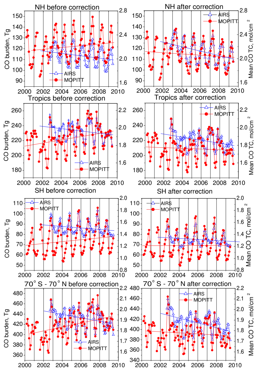
Fig. 7. Effect of correction for four latitudinal belts. Monthly mean CO burdens in Tg for latitudinal belts: 30° N–70° N (NH), 30° S–30° N (Tropics), 30° S–70° S (SH) before (left) and after (right) correction obtained from comparison with ground-based instruments. The right-side scale corresponds to mean TC in 10^{18} molecules \text{cm}^{-2} . Red and blue straight lines are linear regressions for MOPITT and AIRS, respectively (see also Table 4).
