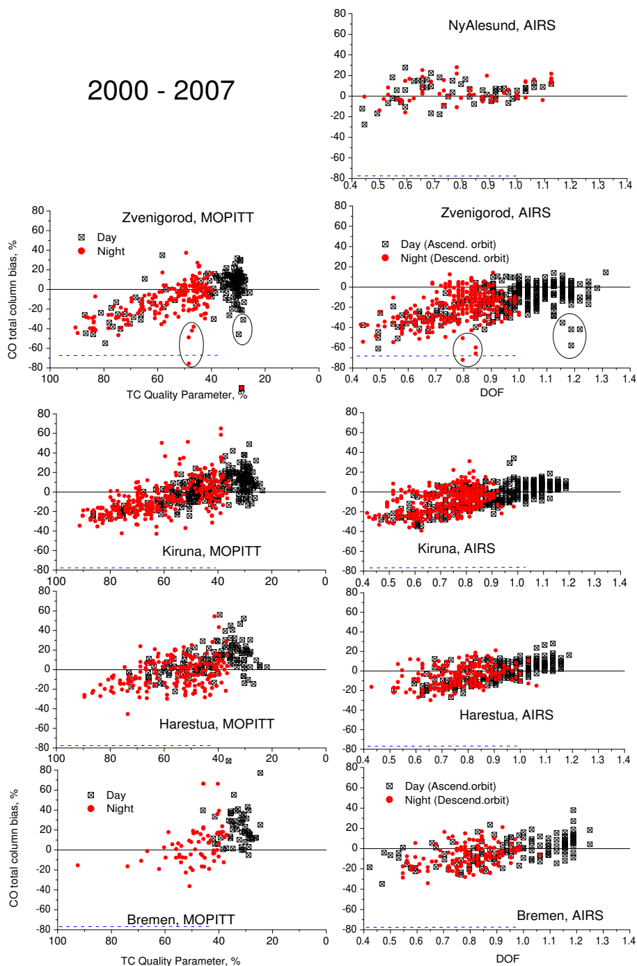
Fig. 2a. MOPITT and AIRS CO TC daily deviations from ground truth (in another words, satellite minus FTS) plotted as a function of information content. Total Column Quality Parameter (TCQP) for MOPITT (note a reverse scale) is the air pressure weighted means of the Profile Percent A priori determined for every grid cell (Yurganov et al., 2008). DOF for AIRS is the number of Degrees of Freedom of the retrieval (McMillan et al., 2009). Encircled symbols correspond to a period of peat fires in August–September 2002 around Zvenigorod (see discussion in the text).
