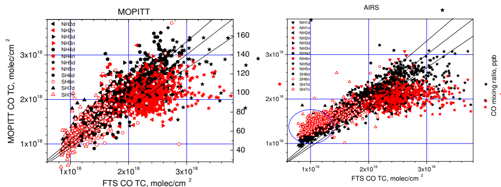
Fig. 4. Scattergrams of daily mean CO TC simultaneously measured by two satellite sounders and six FTS (MOPITT case) or seven FTS (AIRS case) for all matching days. Lines of equal TC and \pm 10\% are shown. Ground-based sites are designated according to Table 1, e.g., NH2d means Kiruna day-time satellite measurements, SH7n means Lauder night-time satellite measurements, etc. Encircled points for AIRS are for the lowest measured TC. Right scales are approximate mean mixing ratios in ppb ( TC/2.15 \times 10^{25} ).
