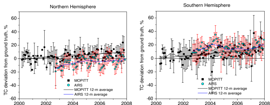
Fig. 5. Temporal stability of two sounders in both hemispheres. Monthly mean deviations of CO TC measured by satellite sounders from those measured by ground-based spectrometers. Vertical bars represent standard deviations (black – MOPITT, red – AIRS). Black and blue lines correspond to 12-month sliding averages; straight lines for MOPITT are linear regressions with slopes (1.4 \pm 0.4)\% per year (NH) and (1.8 \pm 0.4)\% per year (SH).
