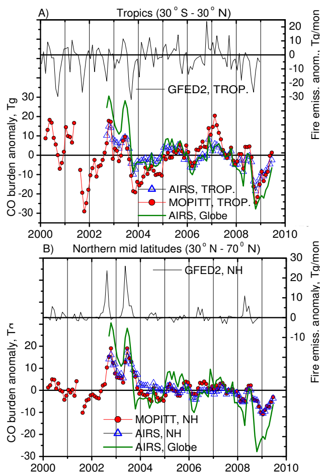
Fig. 11. CO burden regional anomalies compared with emission from biomass burning. (A) Top panel: anomalies of CO emission from biomass burning according to GFED2. Bottom panel: anomalies of CO burden for the tropical belt measured by the two satellite sounders as corrected in Sect. 2. The anomalies of global burden are shown for comparison. (B) The same as in (A), but for Northern mid-latitudes.
