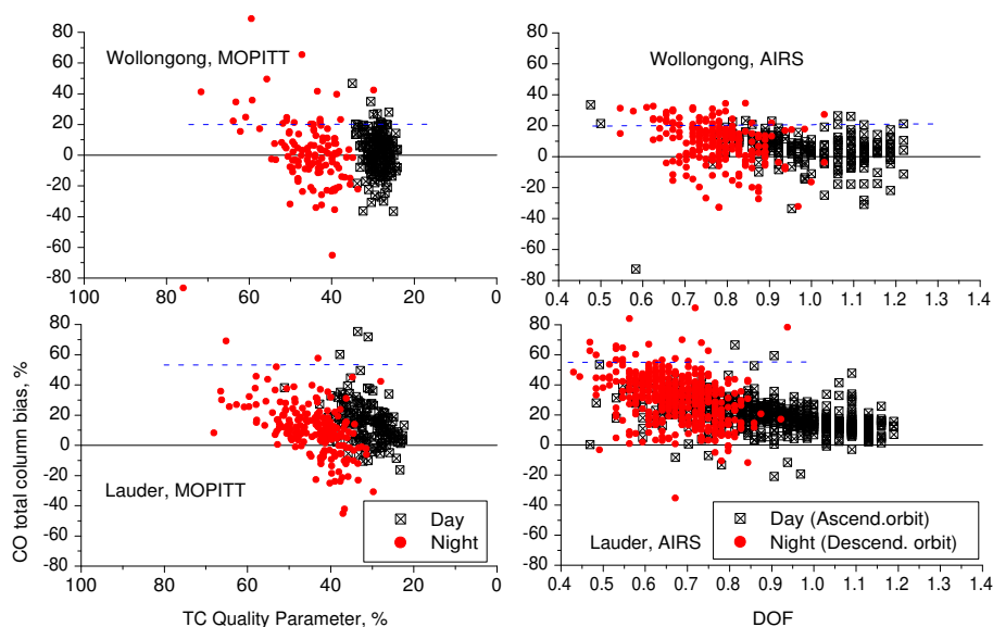
Fig. 2b. The same as Fig. 2a, but for the Southern Hemisphere.
