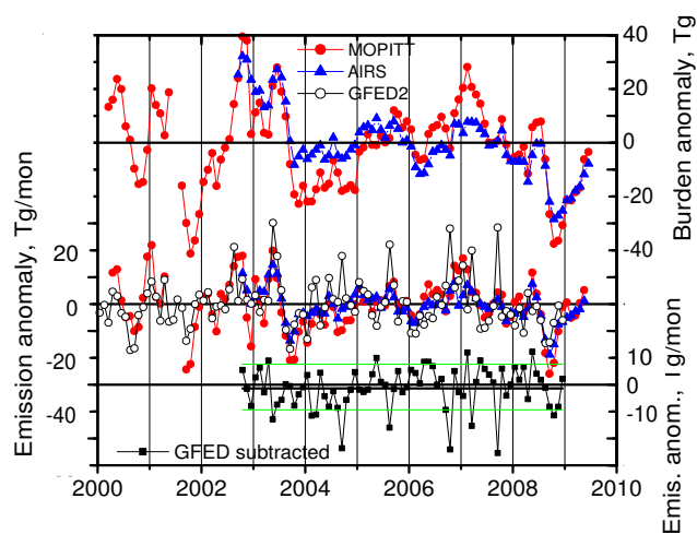
Fig. 10. Global CO emission anomalies derived from MOPITT and AIRS data and compared to GFED2. Top panel, right-hand scale: Anomalies of global ( 70^{\circ} S to 70^{\circ} N) monthly mean CO burden observed by the two satellite sounders. Middle panel, left-hand scale: Anomalies of monthly mean CO global emissions calculated from burden anomalies assuming the reaction with OH is the only sink for CO and [OH] according to Spivakovsky et al. (2000). Bottom panel, right-hand scale: Averaged MOPITT and AIRS emission anomalies minus fire CO emission anomalies from GFED2, representing all other changes except wild fires. Straight green lines correspond to \pm STD.
