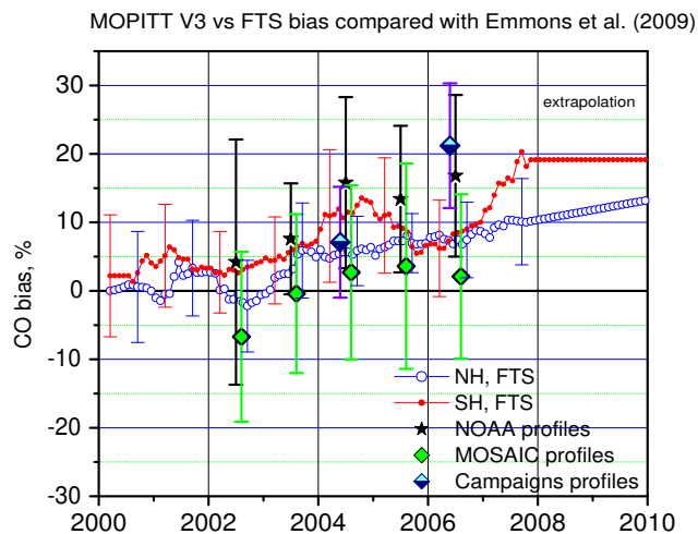
Fig. 6. CO TC bias used as MOPITT V3 correction factor in comparison with other validation results. The MOPITT bias vs. FTS is a sliding average of monthly means until December 2007 and an extrapolation thereafter. Emmons et al. (2009) validation results are plotted for comparison.
