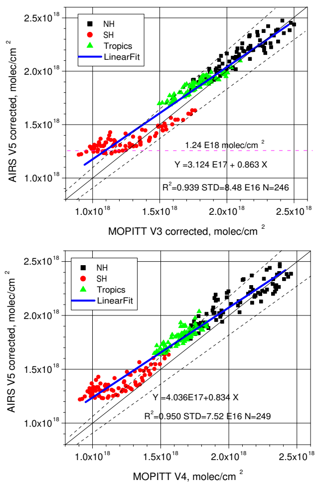
Fig. 9. Comparison of monthly mean CO TC measured by AIRS (V5 corrected) and by MOPITT (V3 corrected and V4) and averaged over mid-latitudes of both hemispheres and over tropics.
