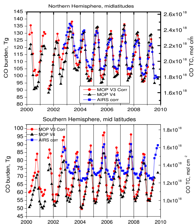
Fig. 8. Comparison of CO total burdens measured by two sounders over the Northern and Southern Hemispheres in the same latitudinal belts as in Fig. 7. Note the general good agreement between our corrected MOPITT V3 and the new MOPITT V4.
