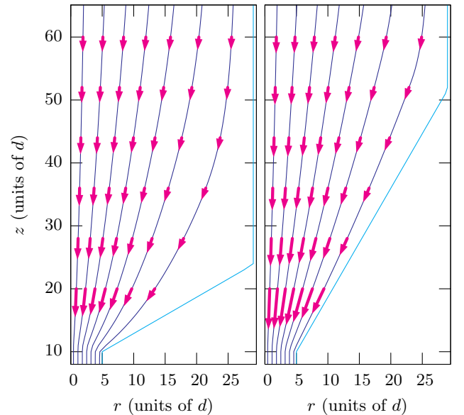
FIG. 4: (Color online) Streamlines of the mean flow in the 30° (left) and 60° reactor geometries for the numerical solution of the Kinematic Model. Arrows are proportional to the velocity vectors in selected horizontal slices.
