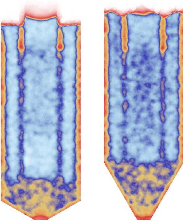
FIG. 7: Plots of local volume fraction ( 1 - \text{porosity} ) in a vertical cross section for the thirty degree reactor geometry (left) and the sixty degree reactor geometry (right), calculated using a Voronoi cell method. Volume fractions of 50%, 57%, 60%, and 63% are shown using the colors of red, yellow, dark blue, and cyan respectively. Colors are smoothly graded between these four values to show intermediate volume fractions. High in the bulk of the container, the packing fraction is approximately 63%, apart from in a small region of lower density at r_{\text{in}} = 14.5d , corresponding to packing defects introduced by the guide ring. In both geometries a sharp reduction in density is observed in a region above the orifice, where particles in the parabolic flow region are forced to undergo local rearrangements.
