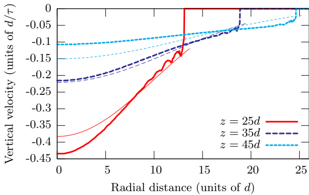
FIG. 5: (Color online) Velocity profiles for the 60^\circ reactor geometry (heavy lines), with a comparison to the Kinematic Model for b = 3d (thin lines).
