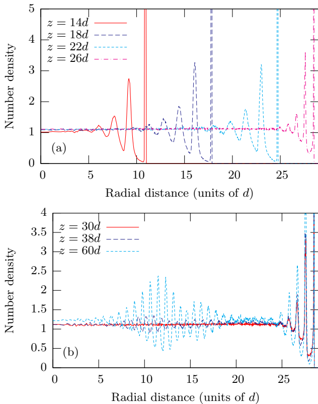
FIG. 9: (Color online) Number density plots in the thirty degree reactor geometry for several low cross sections (a), and several high cross sections (b).
