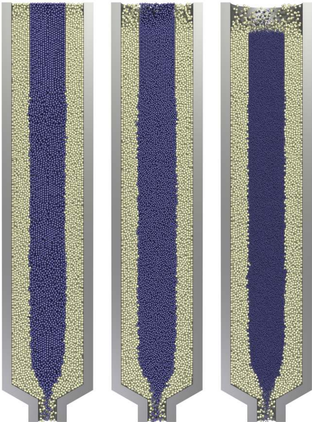
FIG. 18: (Color online) Snapshots of vertical cross-sections for the bidisperse simulations. From left to right, the moderator pebbles have diameters 1d , 0.8d , and 0.5d while the fuel pebbles are of constant size 1d .
