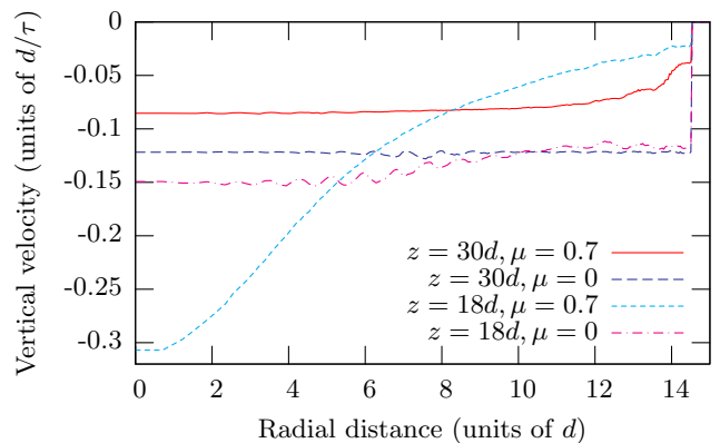
FIG. 15: (Color online) Comparison of velocity profiles for simulations with and without wall friction for two different heights.
