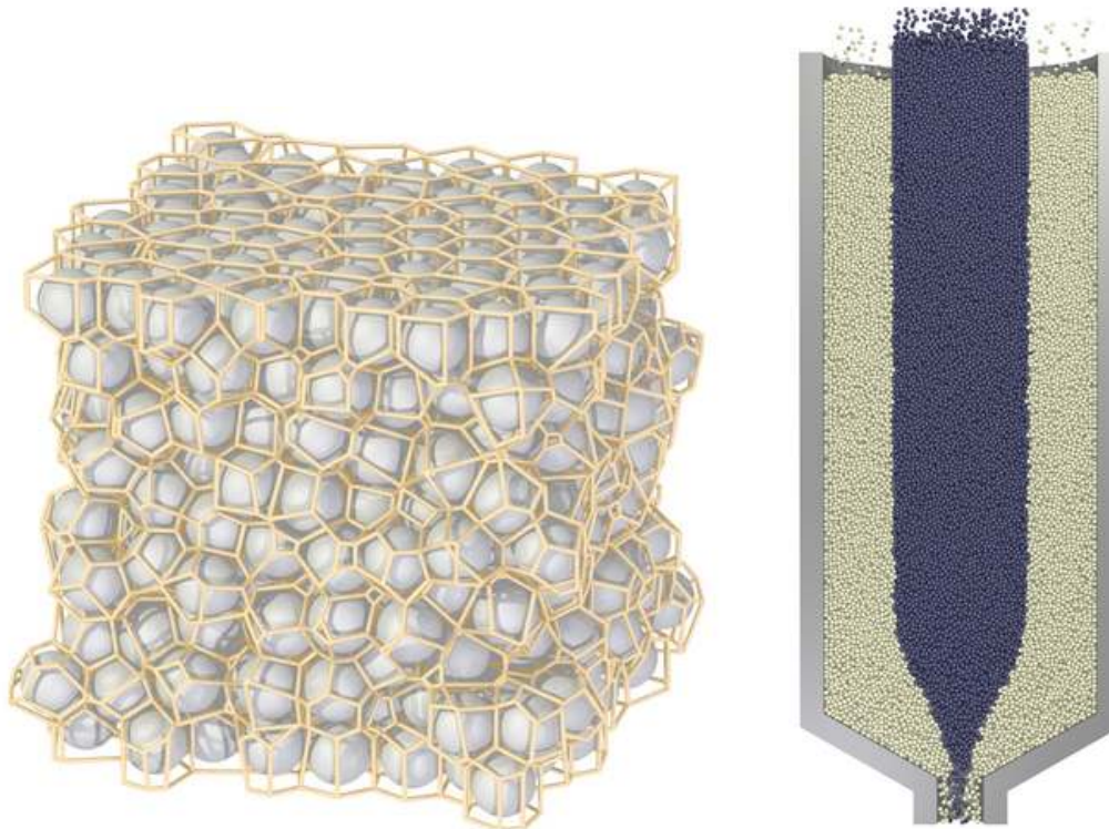
Fig. 3. Voronoi tessellation of a flowing random packing.
