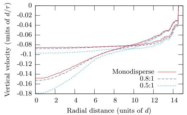
FIG. 19: (Color online) Comparison of velocity profiles for the three bidisperse simulations. The three flatter curves are calculated at z = 30d in the plug-like flow region while the other three were taken at z = 22d in the parabolic flow region.
