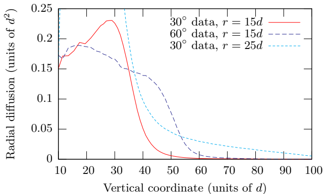
FIG. 6: (Color online) Radial diffusion of particles about streamlines of the mean flow as a function of height, z , in both reactor geometries for pebbles starting at z = 110d in an annulus of radius r = 15d , at the edge of the dynamic central column in MPBR. For the 30^\circ geometry, we also show data for pebbles near the wall at r = 25d .
