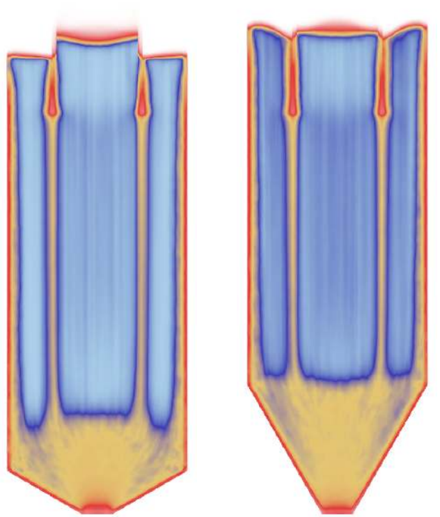
FIG. 8: Time-averaged plots of the local volume fraction, using the same color scheme as figure 7.
