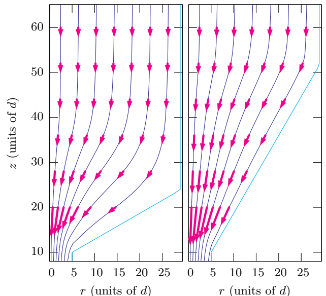
FIG. 2: (Color online) Computed streamlines of the mean flow in the 30^\circ (left) and 60^\circ reactor geometries. Arrows are proportional to the velocity vectors in selected horizontal slices.
