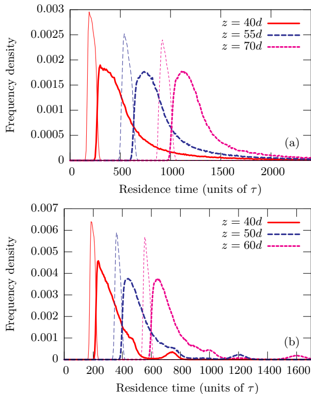
FIG. 11: (Color online) Residence-time probability densities for the time it takes particles to drop from a specific height z out of the container, for the thirty degree reactor geometry (a) and sixty degree reactor geometry (b) for fuel pebbles (heavy lines) and for moderator pebbles (thin lines).
