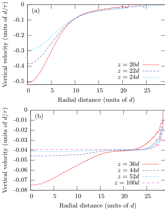
FIG. 3: (Color online) Velocity profiles for the thirty degree reactor geometry for several low cross-sections (a) and several high cross-sections (b).
