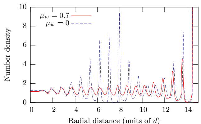
FIG. 16: (Color online) Comparison of number density profiles at z = 60d for simulations with and without wall friction.
