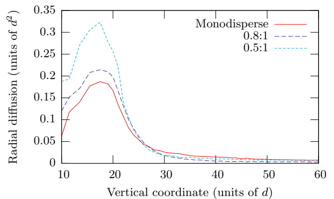
FIG. 20: (Color online) Comparison of particle diffusion for the three bidisperse simulations.
