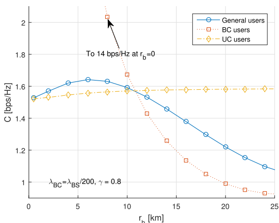
FIGURE 5. Spectral efficiency versus the BC radius.
