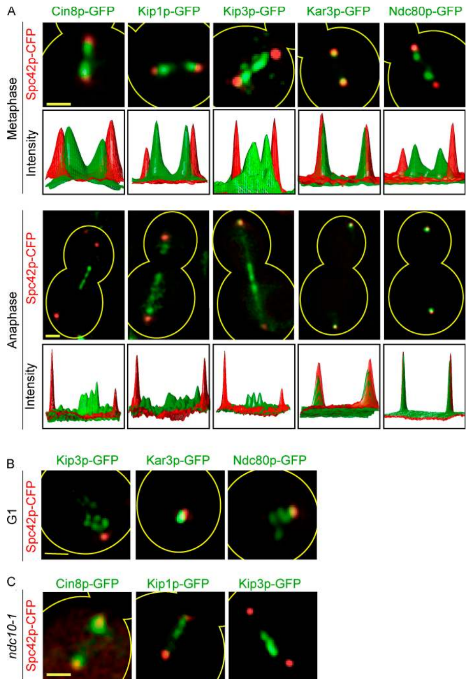
Figure 1. Localization of GFP-tagged kinases in wild-type cells. (A) Typical 2D projections of 3D images showing metaphase (top) and anaphase (bottom) cells coexpressing the SPB marker Spc42p-CFP (red) and Cin8p-GFP, Kip1p-GFP, Kip3p-GFP, Kar3p-GFP, or Ndc80p-GFP (green). Surface plots beneath each image depict fluorescence signal intensity distribution in arbitrary units for CFP (red) and GFP (green). The intensity distributions were generated from 2D summed projections of 3D image stacks. Intensities are not comparable between images. (B) Representative 2D projections of 3D images of G1 cells coexpressing Kip3p-GFP, Kar3p-GFP, or Ndc80p-GFP (green) with Spc42p-CFP (red). (C) Images of cells expressing Cin8p-GFP, Kip1p-GFP, and Kip3p-GFP (green) with Spc42p-CFP (red) in ndc10-1 cells. Strains were grown to midlog phase at 25°C and shifted to 37°C for 3 h before analysis. Spindles elongate abnormally in many ndc10-1 cells, creating metaphase cells with spindles lengths that are typical of anaphase (>2.0-μm long). Bars, 1 μm.
