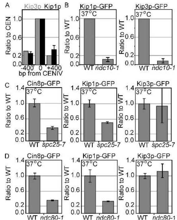
Figure 3. Dependence of kinesin-CEN cross-linking by ChIP on core kinetochore components. (A–D) ChIP of Kip1p-GFP, Kip3p-GFP, and Cin8p-GFP to CENIV or flanking DNA as assayed in wild-type (A), ndc10-1 (B), spc25-7 (C), or ndc80-1 (D) cells. Asynchronous cultures were grown to midlog phase at 25°C and shifted to 37°C for 3 h (B–D) before analysis. (A) Results are expressed as the ratio of the percentage of immunoprecipitation from the arm regions to the percentage of immunoprecipitation of the CEN . (B–D) Results are expressed as a ratio of the percentage of immunoprecipitation in the mutant to the percentage of immunoprecipitation of the wild-type strain. Error bars represent the SEM. n = 2 .
