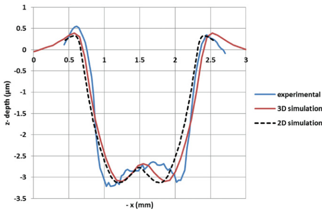
Figure 9. Surface deformation induced by a single 1.6 mm laser impact on 2050-T8—experimental versus numerical data ( I_0 = 5.5 \text{ GW cm}^{-2} )—2D and 3D simulations using a spherical P = f(x, y) distribution with P_0 = 3.8 \text{ GPa} .
