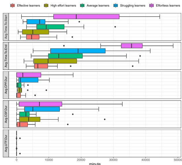
FIGURE 9. Boxplots indicating homework time of five groups.
