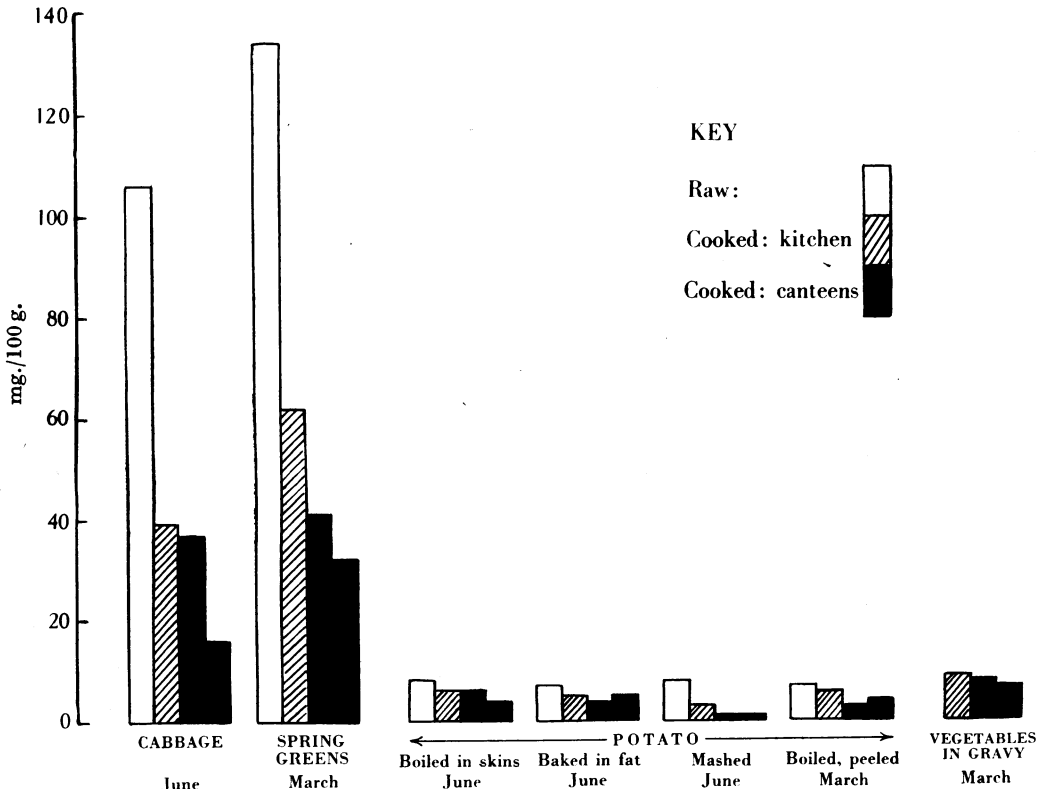
Fig. 1. Effect of cooking and transit on vitamin C content of vegetables.
