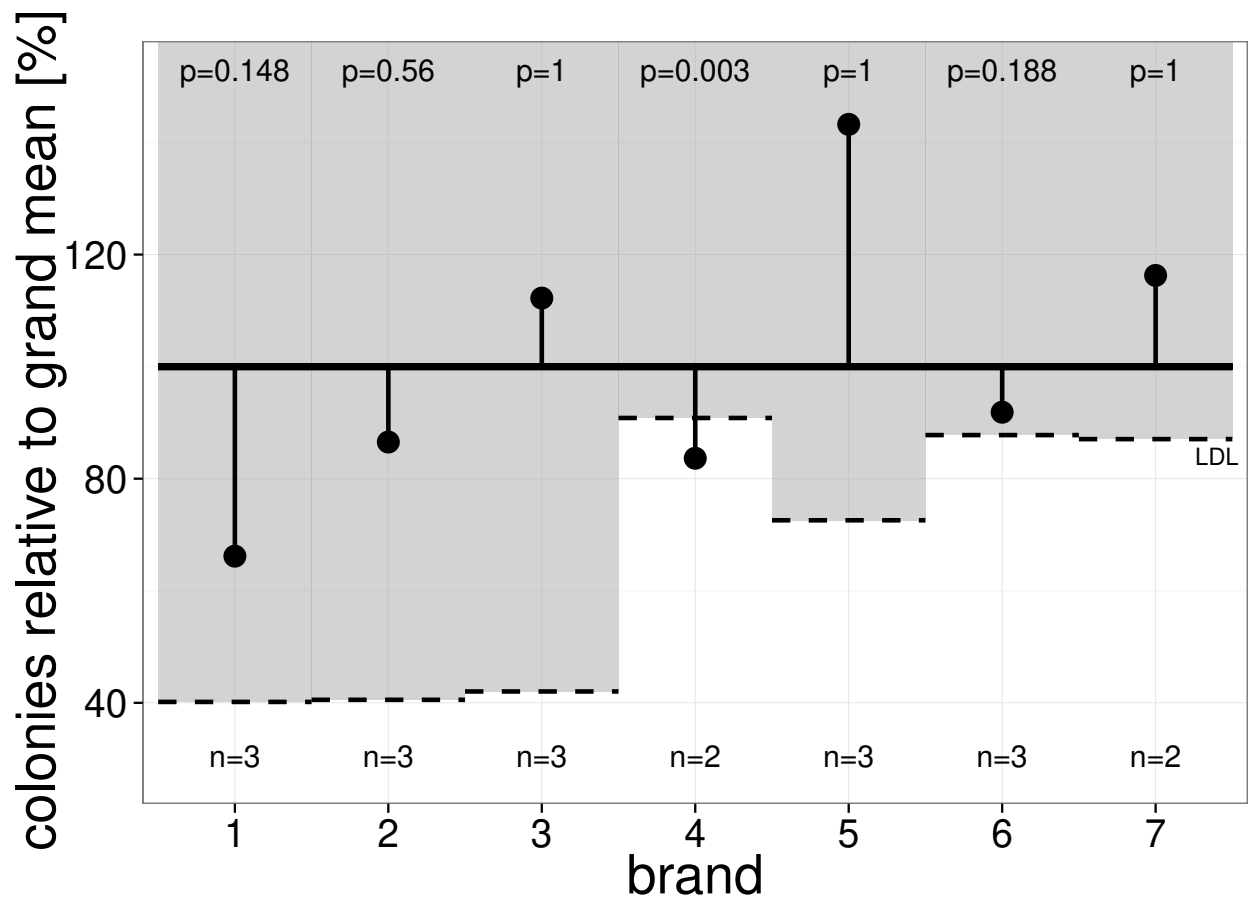
Figure 6: ANOM decision chart for the water filter data (accounting for heterogeneous variances using multiple degrees of freedom) in terms of percentages.
