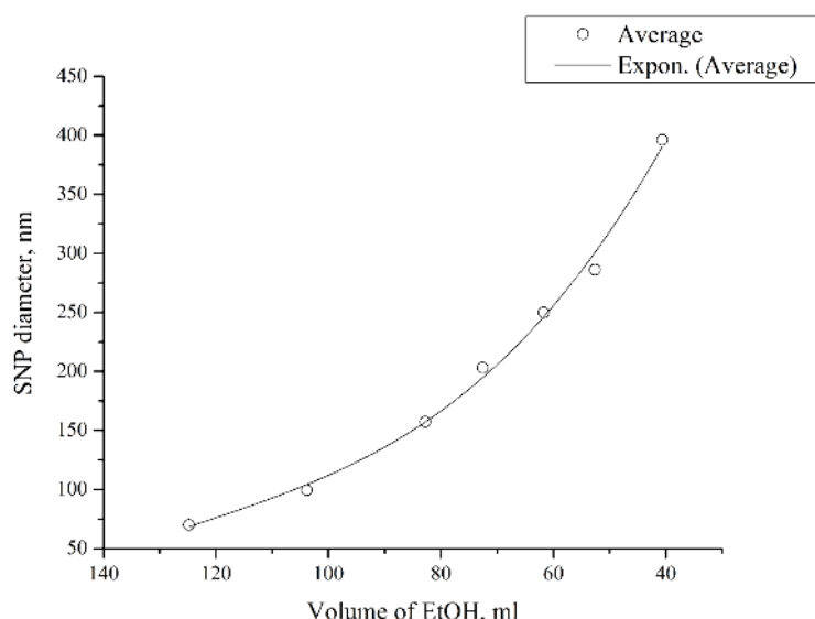
Fig. 11. Influence of the solvent content on the particle size of the Stober reaction product according to the data of [48]
