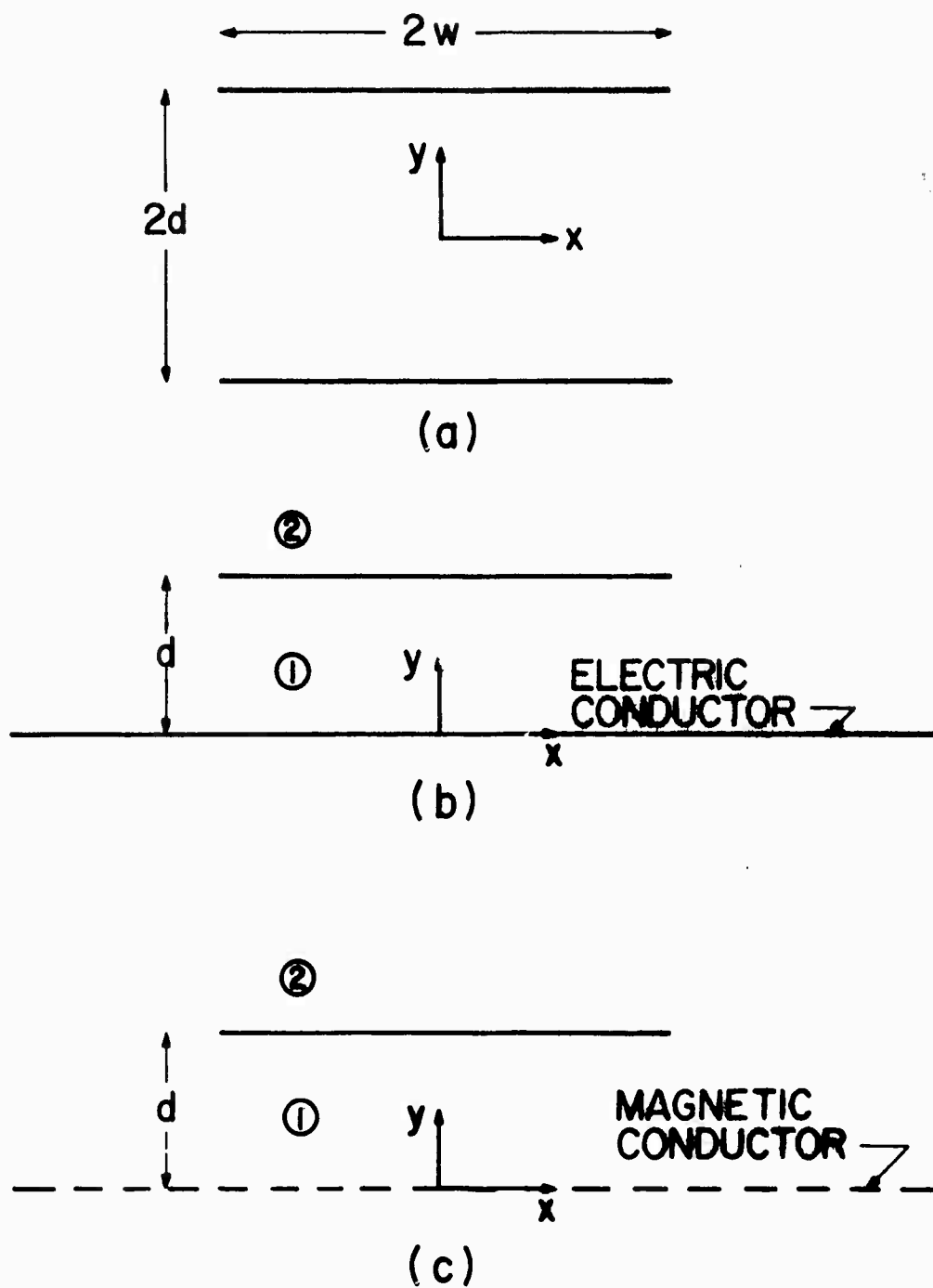
Figure 1. (a) Cross Section of a Finite-Width Parallel-Plate Waveguide (b), (c) Equivalent Structure.
