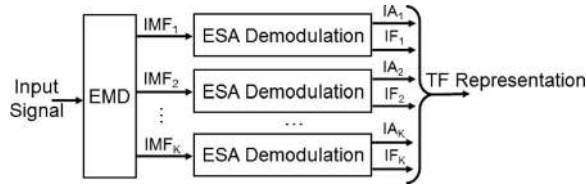
Fig. 1. Block diagram of TH transform.
