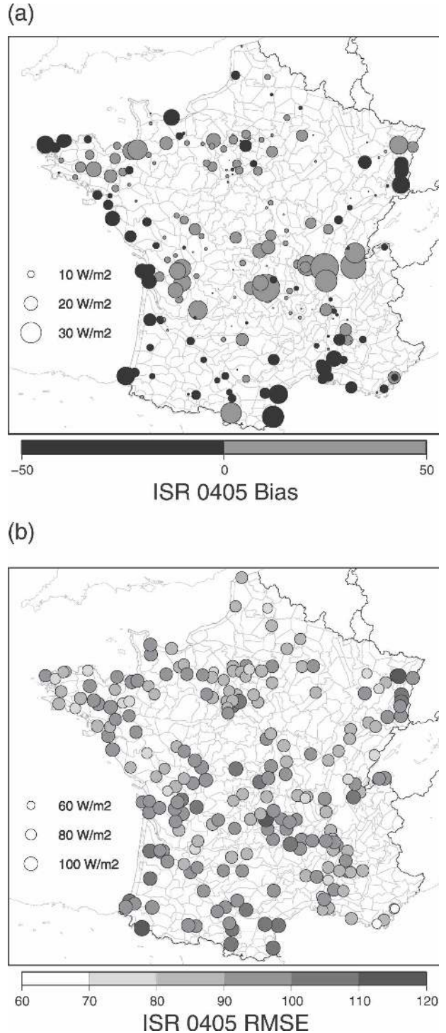
FIG. 9. Comparison of the analyzed and observed mean incoming solar radiation ( W m^{-2} ) for 2004/05 at the points of observation. (a) The bias, and (b) the RMSE. The size of the circles is proportional to the magnitude of the bias or RMSE.
