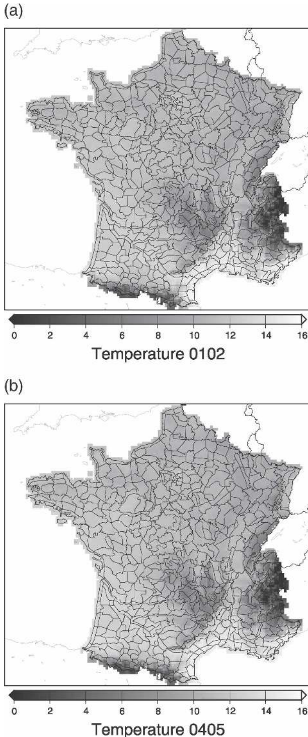
FIG. 3. Analyzed mean temperature (°C) for the (a) 2001/02 and (b) 2004/05 on a grid of 8-km resolution. The analysis has been calculated using data from 1062 stations. The thin lines correspond to the borders of the climatically homogeneous zones.
