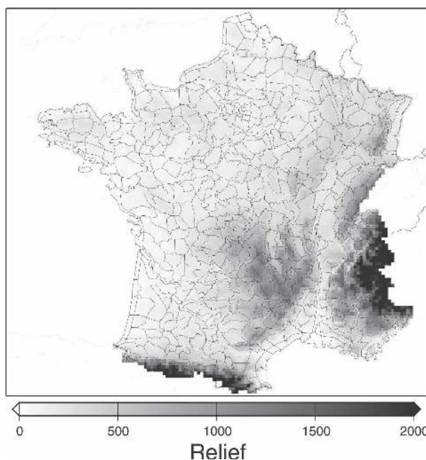
FIG. 1. Relief (m) of France on the grid of 8-km resolution used by SAFRAN/F. The thin black lines are the borders of the climatologically homogeneous zones used by SAFRAN/F.
