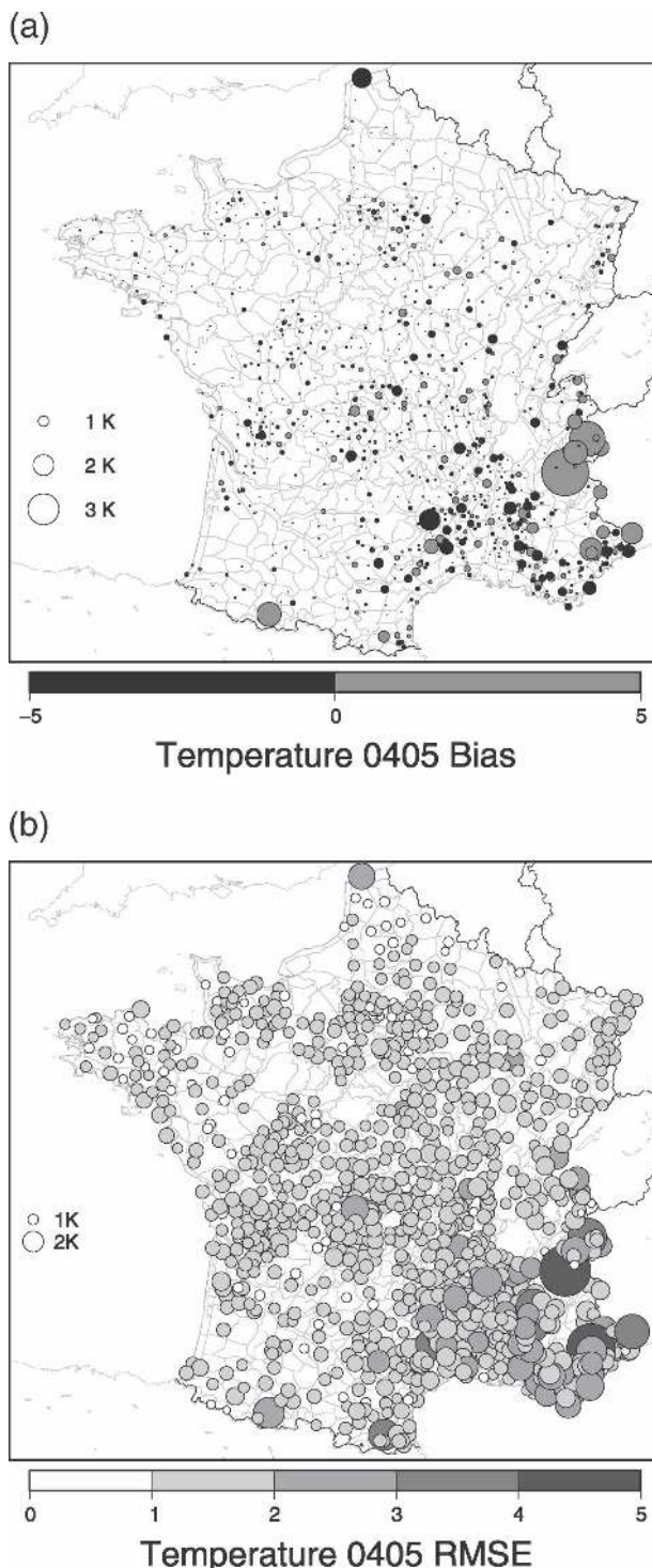
FIG. 2. Comparison of the analyzed and observed mean temperatures ( ^{\circ}\text{C} ) for the hydrological year 2004/05 at the points of observation. (a) The bias, and (b) the RMSE. The size of the circles is proportional to the magnitude of the bias or RMSE.
