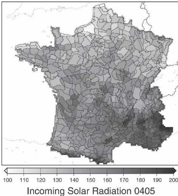
FIG. 8. Analyzed mean incoming solar radiation ( W m^{-2} ) for 2004/05 on a grid of 8-km resolution. Because of the low number of observations (239 stations), this field is not analyzed but is calculated using a radiation scheme. The thin lines correspond to the borders of the climatically homogeneous zones.
