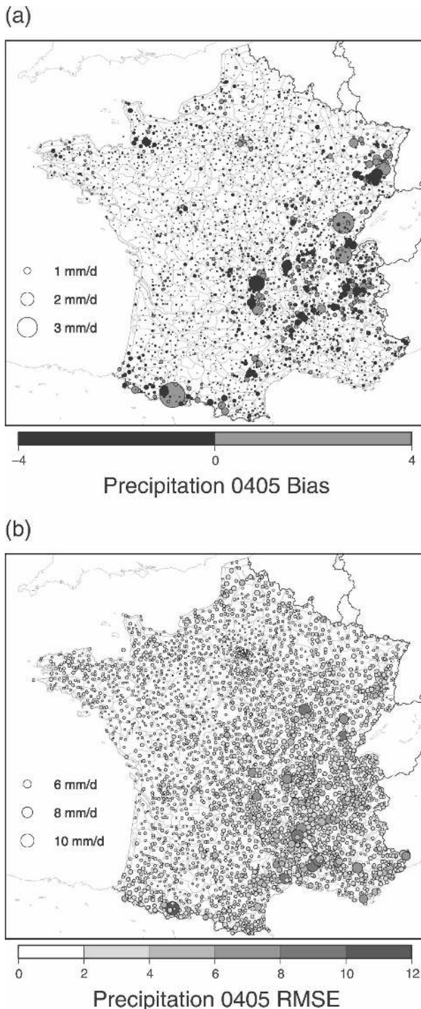
FIG. 11. Comparison of the analyzed and observed mean precipitation rates ( \text{mm day}^{-1} ) for 2004/05 at the points of observation. (a) The bias, and (b) the RMSE. The size of the circles is proportional to the magnitude of the bias or RMSE.
