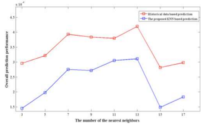
Fig. 6. Overall prediction performances with different settings of k in the proposed k-NN based method
