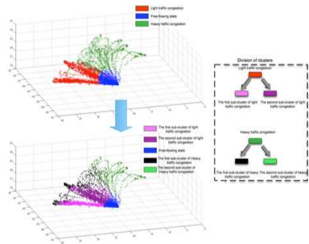
Fig. 4. Division of clusters after increasing the number of cluster
