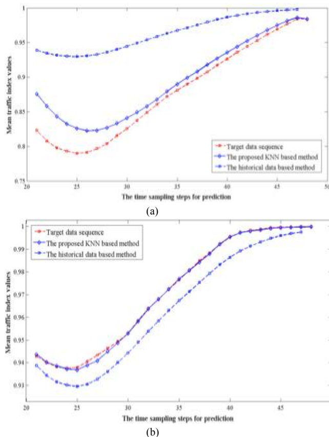
Fig. 7. (a) (b) Comparison of prediction performances on two different traffic scenes
