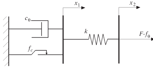
Fig. 10. Rheological structure of a MR damper for the Bingham body model
