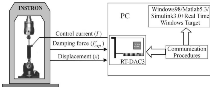
Fig. 16. Scheme of the experimental setup for examinations of a MR linear damper
