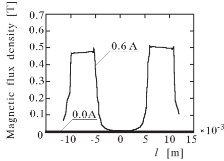
Fig. 6. Distribution of magnetic flux density along the gap for I = 0.0 A and I = 0.6 A
