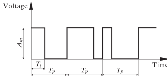
Fig. 5. Pulse width modulation
