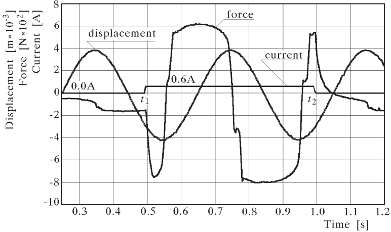
Fig. 8. Displacement vs. time; curen in the coil vs. time; damping force vs. time
