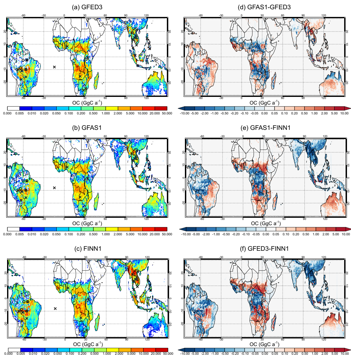
Figure 1. (a–c) Total annual emissions of organic carbon (OC) in \text{GgC a}^{-1} averaged over the period of January 2003 to December 2011 from (a) GFED3, (b) GFAS1 and (c) FINN1. Black circles mark the locations of the four aerosol measurement stations and black crosses mark the locations of the 27 AERONET stations (see Table S1). (d–f) Absolute difference in 2003–2011 mean annual OC emissions between GFAS1, GFED3 and FINN1, (d) GFAS1 minus GFED3 (e), GFAS1 minus FINN1, and (f) GFED3 minus FINN1. The FINN1 OC emissions (with a 1 \text{ km} \times 1 \text{ km} horizontal resolution) were aggregated onto a grid of 0.5^\circ \times 0.5^\circ resolution to compare with GFED3 and GFAS1.
