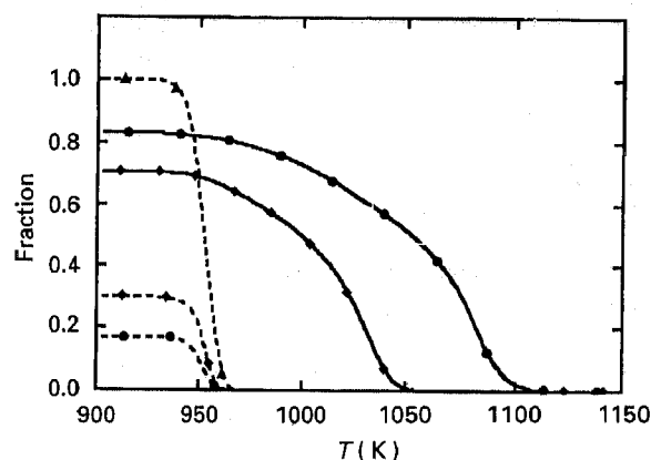
Figure 4 Calculated fractions of pro-eutectoid ferrite and pearlite as a function of the temperature for Fe-0.17 mass % C, Fe-0.36 mass % C and Fe-0.8 mass % C alloys at a cooling rate of 20 K min -1 . ● x^{\alpha, \text{pro}} (0.17 mass % C); —●— x^P (0.17 mass % C); —◆— x^{\alpha, \text{pro}} (0.36 mass % C); —◆— x^P (0.36 mass % C); —▲— x^P (0.8 mass % C).
