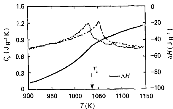
Figure 1 The measured heat capacity for ferrite C_p^f in pure iron. The experiments were performed at a scanning rate of 20 \text{ K min}^{-1} . Also the enthalpy difference between ferrite and austenite is given as a function of temperature (solid line).
