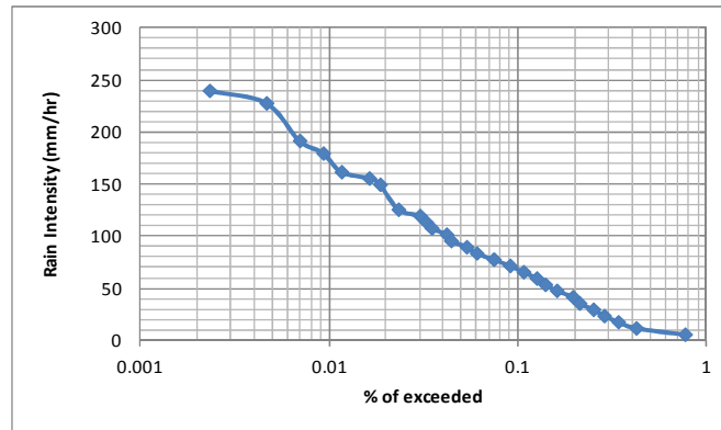
Fig. 3: One month rain intensity (mm/hr) as a % of time exceeded measured on July 2011.
