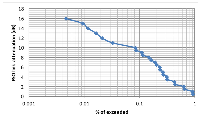
Fig. 4: One month rain attenuation on FSO link (dB) as a % of time exceeded measured on July 2011.
