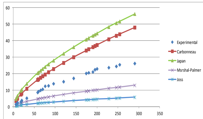
Fig. 5: Comparison of measured rain attenuation and that predicted by prediction models using measured rain intensity.
