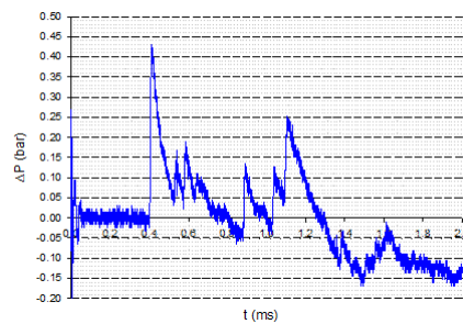
Fig. 34 Time-evolution of pressure - Sensor B - Walls 1 + 2 + 3 + 4
