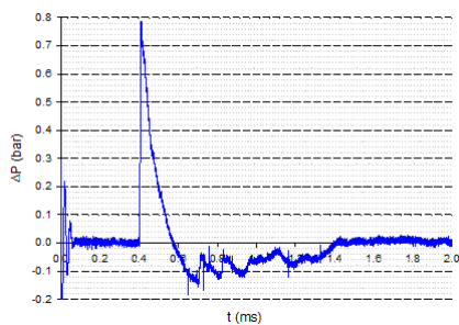
Fig. 4 Pressure-time history - Sensor A - Wall 1 alone
