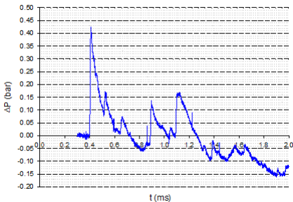
Fig. 32 Pressure-time history - Sensor B Walls 1 + 2 + 3
