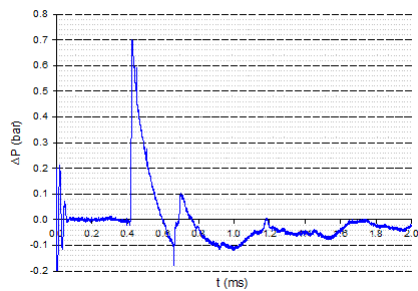
Fig. 11 Pressure-time history - Sensor A - Walls 1 + 4
