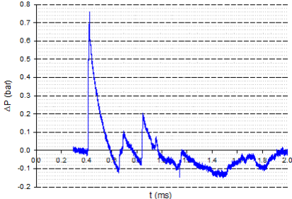
Fig. 15 Pressure-time history - Sensor A Walls 1+ 2+ 4
