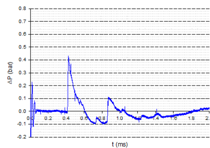
Fig. 5 Pressure-time history - Sensor A - Wall 2 alone
