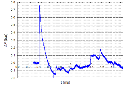
Fig. 10 Pressure-time history - Sensor A - Walls 1 + 3
