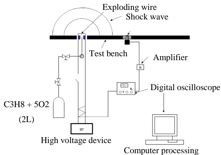
Fig. 1 Experimental setup
