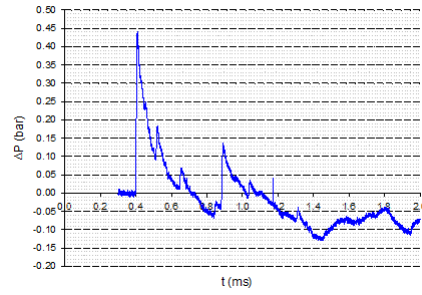
Fig. 25 Pressure-time history - Sensor B - Walls 1 + 3
