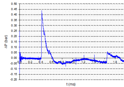
Fig. 36 Pressure-time history - Sensor C - Wall 2
