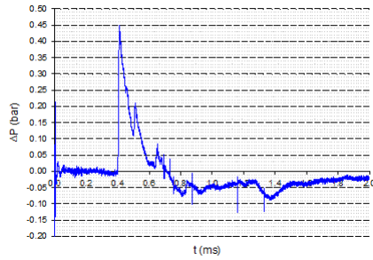
Fig. 20 Pressure-time history - Sensor B - Wall 1 alone
