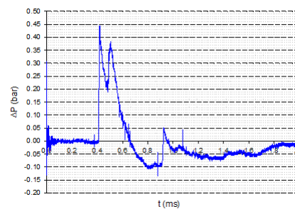
Fig. 38 Pressure-time history - Sensor C - Wall 4
