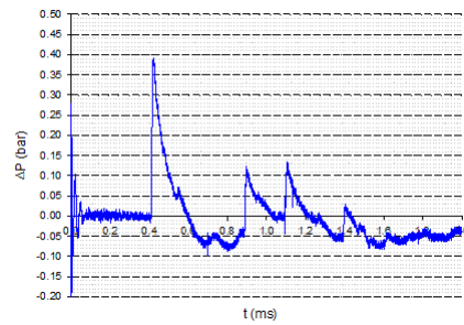
Fig. 27 Pressure-time history - Sensor B - Walls 2 + 3
