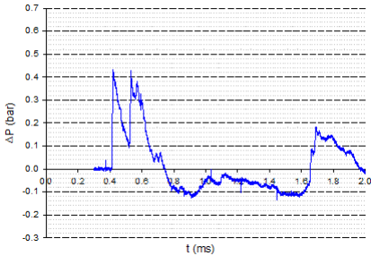
Fig. 47 Time-evolution of pressure - Sensor C Walls 1 + 2 + 3
