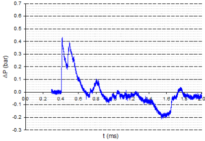
Fig. 45 Time-evolution of pressure - Sensor C Walls 1 + 2 + 4
