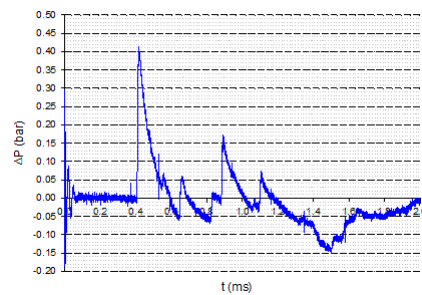
Fig. 29 Pressure-time history - Sensor B - Walls 3 + 4
