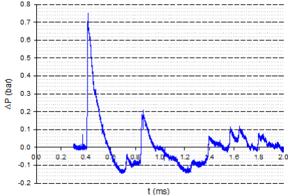
Fig. 16 Pressure-time history - Sensor A Walls 1+ 2+ 3
