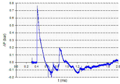
Fig. 9 Pressure-time history - Sensor A - Walls 1 + 2
