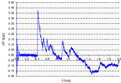
Fig. 31 Pressure-time history - Sensor B Walls 1 + 3 + 4
