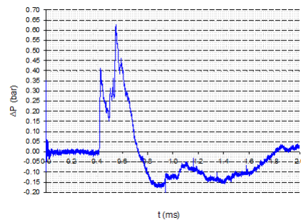
Fig. 44 Pressure-time history - Sensor C - Walls 3 + 4
