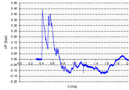
Fig. 40 Pressure-time history - Sensor C - Walls 1 + 3
