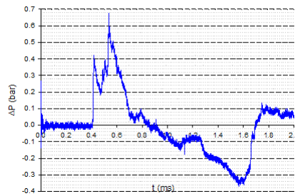
Fig. 49 Time-evolution of pressure - Sensor C – Walls 1 + 2 + 3 + 4
