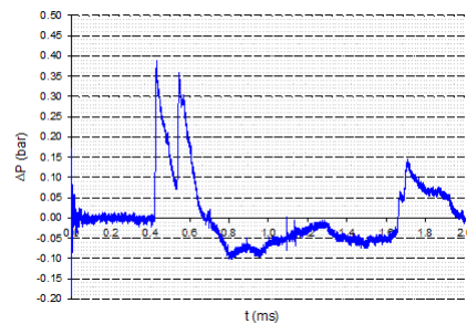
Fig. 42 Pressure-time history - Sensor C - Walls 2 + 3
