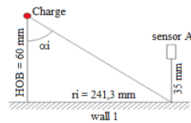
Fig. 8 Configuration for calculation of the Mach stem along Wall 1 - Top view - HOB = Height of burst
