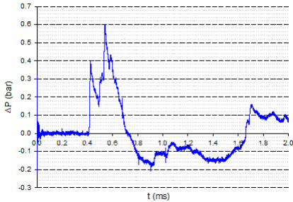
Fig. 48 Time-evolution of pressure - Sensor C Walls 2 + 3 + 4
