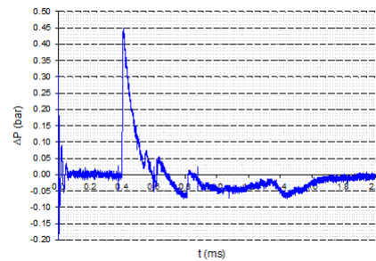
Fig.23 Pressure-time history - Sensor B - Wall 4 alone
