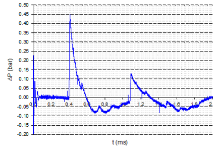
Fig.21 Pressure-time history - Sensor B - Wall 2 alone
