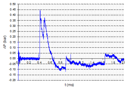
Fig. 43 Pressure-time history - Sensor C - Walls 2 + 4
