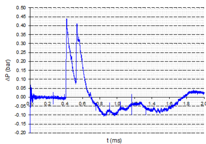
Fig. 327 Pressure-time history - Sensor C - Wall 3
