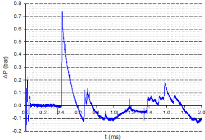
Fig. 17 Pressure-time history - Sensor A Walls 1+ 4+ 3
