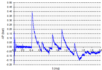
Fig. 33 Pressure-time history - Sensor B Walls 2 + 3 + 4
