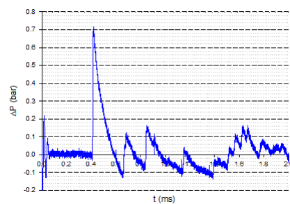
Fig. 19 Pressure-time history - Sensor A - Walls 1 + 2 + 3 + 4
