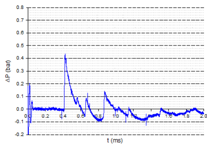
Fig. 13 Pressure-time history - Sensor A - Walls 2 + 4
