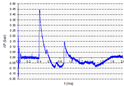
Fig. 22 Pressure-time history - Sensor B - Wall 3 alone
