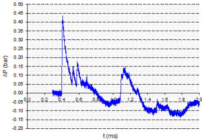
Fig. 30 Pressure-time history - Sensor B Walls 1 + 2 + 4
