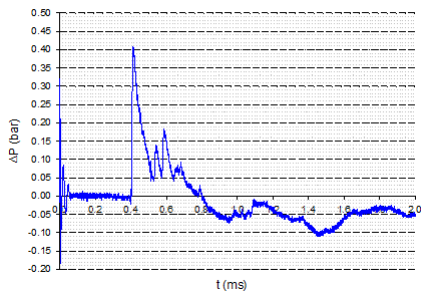
Fig. 26 Pressure-time history - Sensor B - Walls 1 + 4
