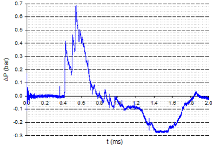
Fig. 46 Time-evolution of pressure - Sensor C Walls 1 + 3 + 4
