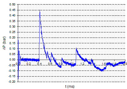
Fig. 28 Pressure-time history - Sensor B - Walls 2 + 4
