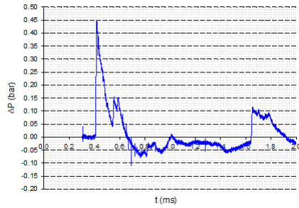
Fig. 39 Pressure-time history - Sensor C - Walls 1 + 2
