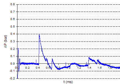
Fig. 14 Pressure-time history - Sensor A - Walls 3 + 4
