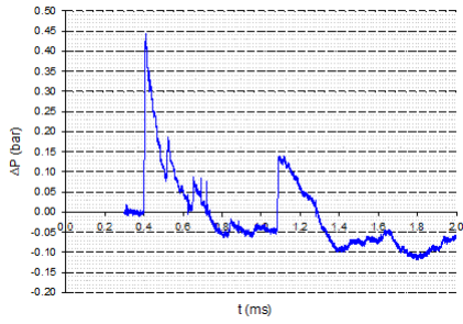
Fig. 24 Pressure-time history - Sensor B - Walls 1 + 2
