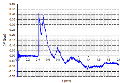
Fig. 41 Pressure-time history - Sensor C - Walls 1 + 4
