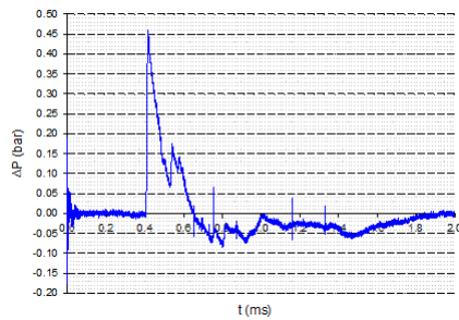
Fig. 35 Pressure-time history - Sensor C - Wall 1
