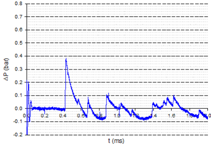
Fig. 18 Pressure-time history - Sensor A Walls 2+ 3+ 4
