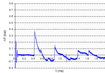
Fig. 12 Pressure-time history - Sensor A - Walls 2 + 3
