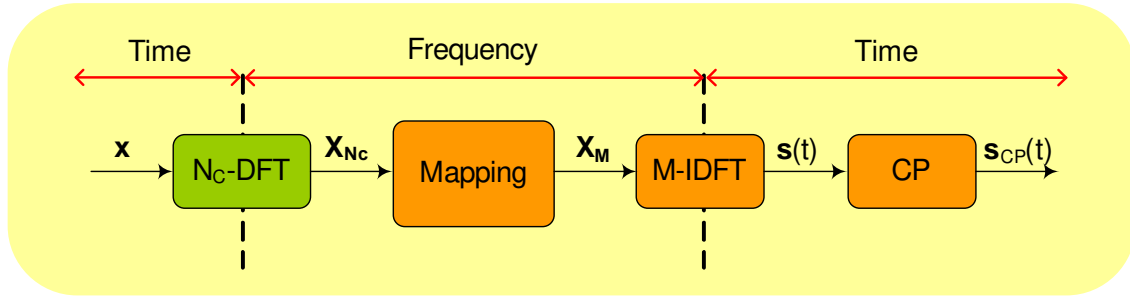
(a) Transmisor SC-FDMA
