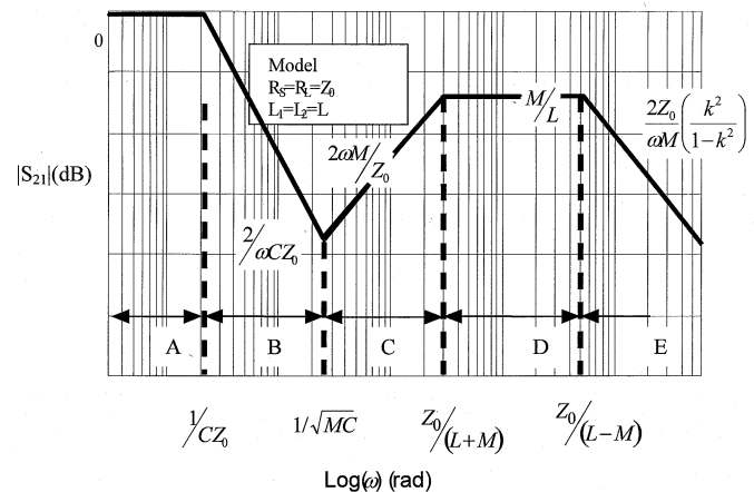
Fig. 2. Bode plot of |S_{21}| of the low-pass filter in Fig. 1.
