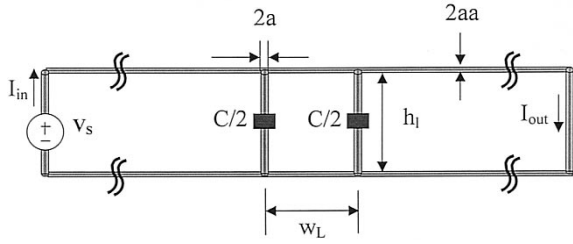
Fig. 13. Model of the two-capacitor filter.
