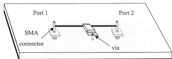
Fig. 3. Test board with a one-capacitor, low-pass filter.
