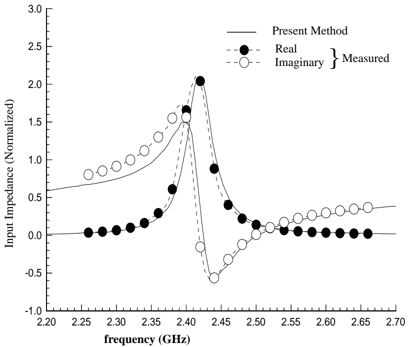
Figure 4 Input impedance of a circular patch ( 2a = 4.11\text{cm} ) loaded with microstrip stub as shown figure 2.
