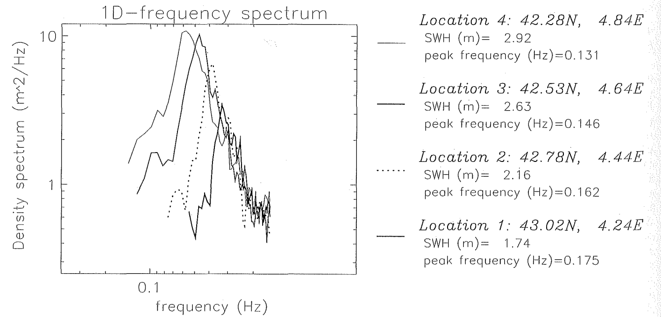
Figure 5. One dimensional spectra obtained from RESSAC at four locations: (1) near the shore in thick solid line, (2) in dotted line, (3) in dash-dotted line, and (4) in open sea in thin solid line. The energy density spectrum is plotted in log-log scale. The horizontal axis is for the frequency (Hz).
