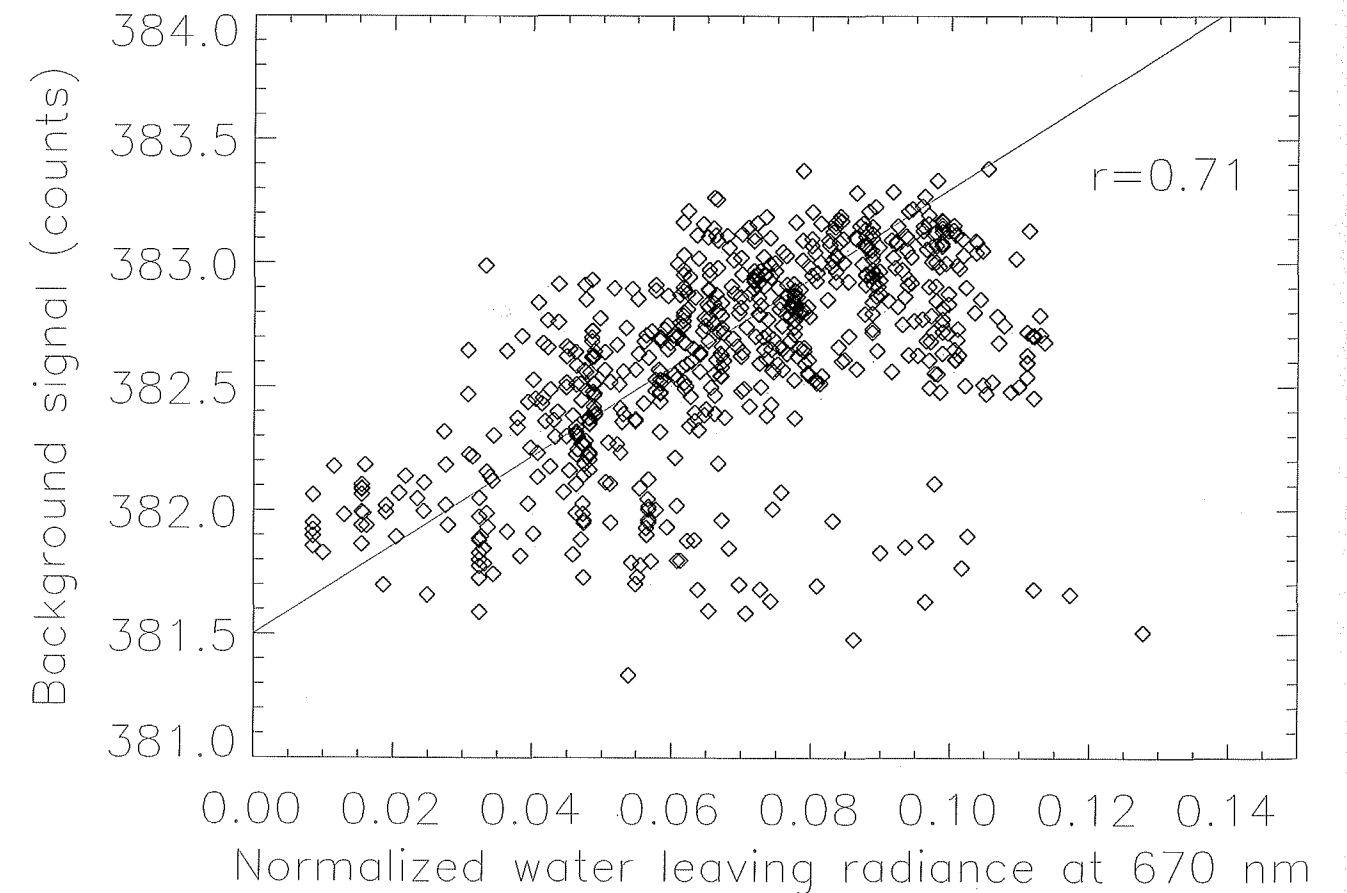
Figure 14. SeaWiFS normalized water leaving radiance at 670 nm versus lidar detected background light at 732 nm.
