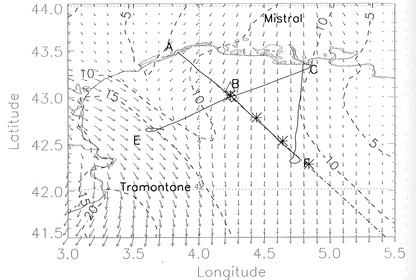
Figure 4. Wind fields simulated in the ABL (at 10 ASL) on 24 March 1998 by the French operational forecast model ALADIN at (a) 1500, (b) 1800 and (c) 2100 UTC. The diamond (triangle) corresponds to the position of the ASIS buoy (Atalante). Superimposed are isotachs between 10 and 20 \text{m s}^{-1} with 5 \text{m s}^{-1} increments. Also superimposed are the ARAT flight tracks corresponding to afternoon flights. The rugged solid line represents the coastline. The asterisks indicate the position of the 1-D spectra shown in Figure 5.
