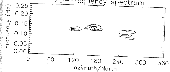
Figure 6. Two dimensional spectra obtained from RESSAC at four locations from the shore to open sea. The normalized energy density (with respect to the peak) is plotted with contour levels of 0.3, 0.5, 0.7, and 0.9. The horizontal axis gives the azimuth (from true North). The vertical axis is for the frequency (Hz). The directions refer to waves going to.
