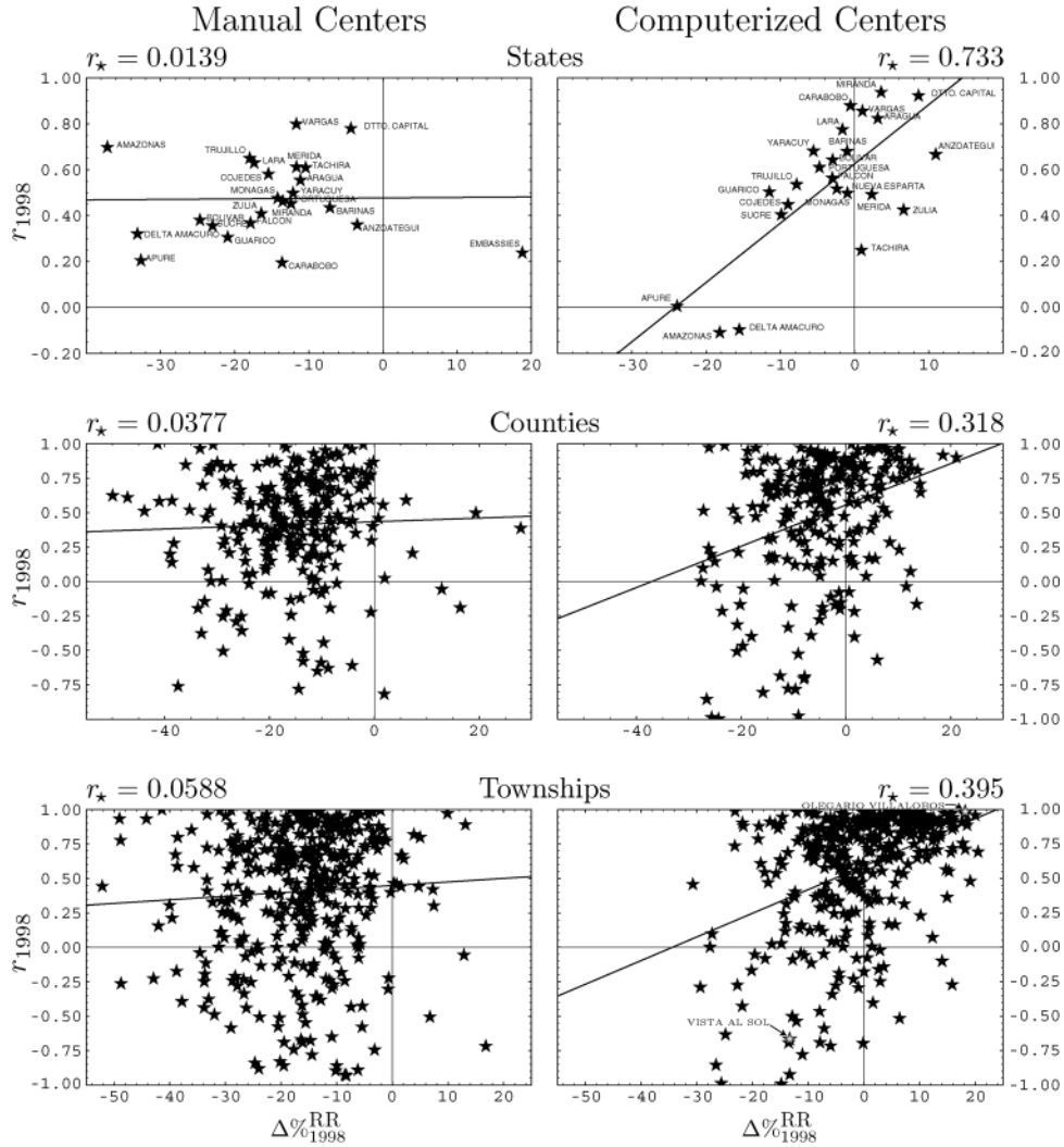
FIG. 10. Relationship between r_{1998} and \Delta\%RR_{1998} at the state, county and township levels for manual and computerized voting centers. The correlation between \Delta\%RR_{1998} and r_{1998} is shown as r_* . Assuming that \Delta\%RR_{1998} and r_{1998} are independent, the probability of seeing those r_* values is calculated in Appendix D.
