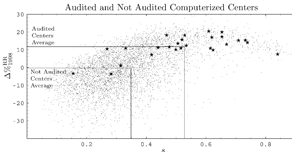
FIG. 14. In this figure, the 26 computerized audited centers are compared with the universe of computerized centers. The average s and \Delta\%_{1998}^{RR} are indicated with lines.
