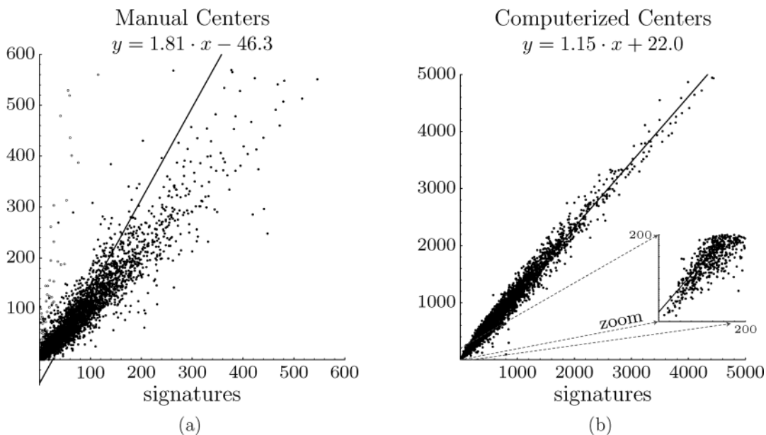
FIG. 6. Manual centers have a correlation of 0.607 with respect to the signatures while computerized centers have a correlation of 0.989. A correlation of 1 would look like a straight line.
