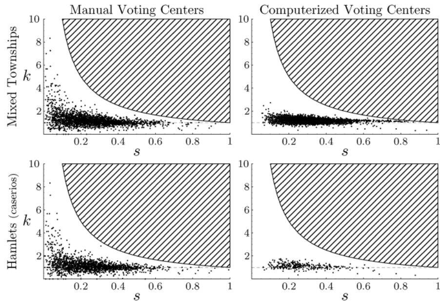
FIG. 5. Relationship between k and s for computerized (right) and manual centers (left) for mixed townships (top) and hamlets (bottom).
