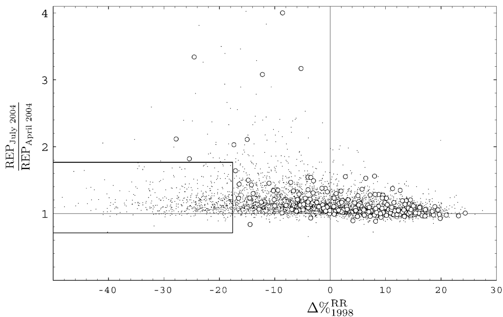
FIG. 25. REP variation versus \Delta\%RR_{1998} in all computerized centers indicating the 192 selected for hot-auditing. None of the 192 selected centers were in the rectangle area.
