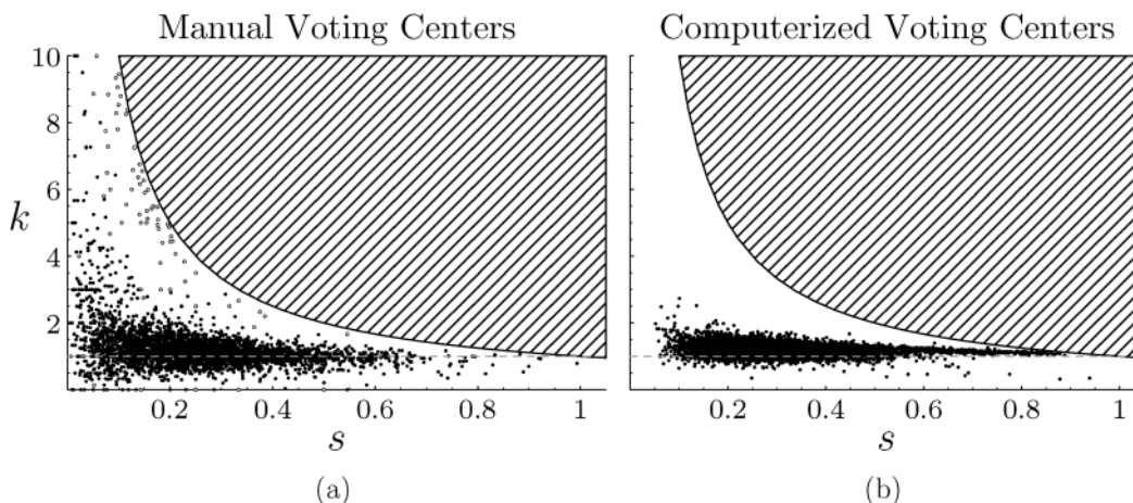
FIG. 3. Relationship between k and s for computerized and manual centers. The shadowed area contains the mathematically impossible values of k . The maximum k value is 1/s . The hollow dots represent voting centers located in consular offices.
