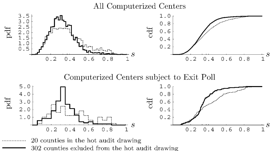
FIG. 21. Comparison of s probability density function (pdf) and cumulative density function (cdf) for computerized centers inside the 20 counties of the hot audit and in the 302 excluded counties.
