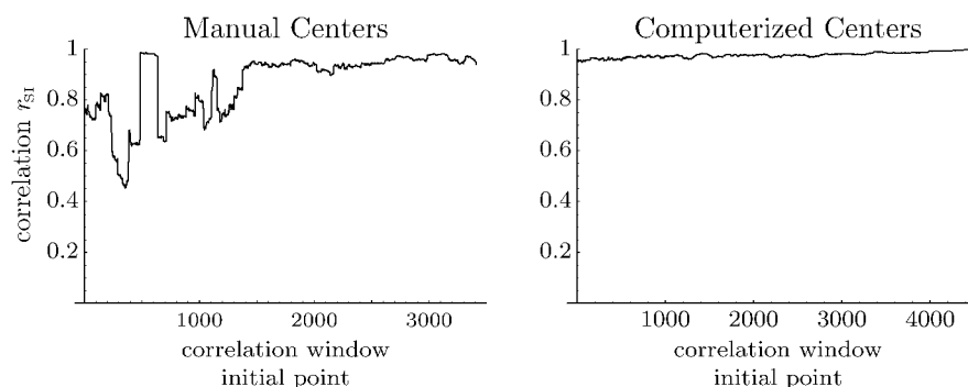
FIG. 7. Correlations plot using a window of 150 voting centers.
