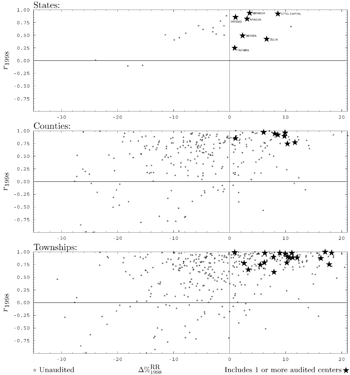
FIG. 15. Townships, counties and states where the 26 audited centers are located. The vertical axis is the correlation with respect to the percentage of opposition in 1998 ( r_{1998} ). The horizontal axis is the difference in percentage of opposition with respect to 1998 ( \Delta\%_{1998}^{RR} ).
