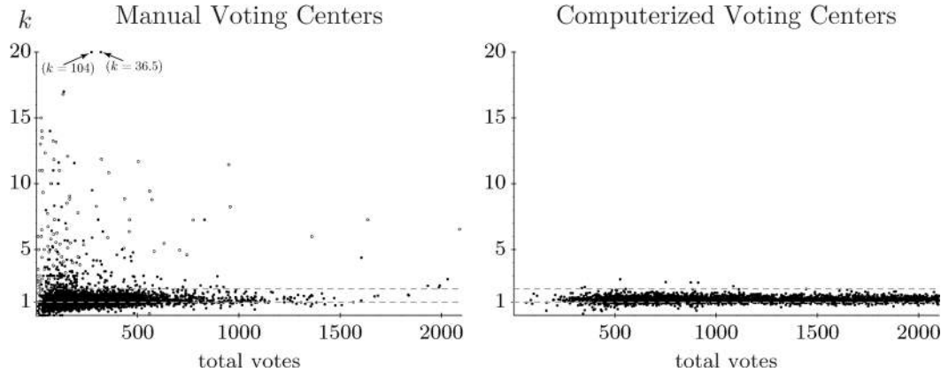
FIG. 4. Relationship between k and total number of votes for computerized and manual centers in the same size range. The hollow dots represent voting centers located in consular offices.
