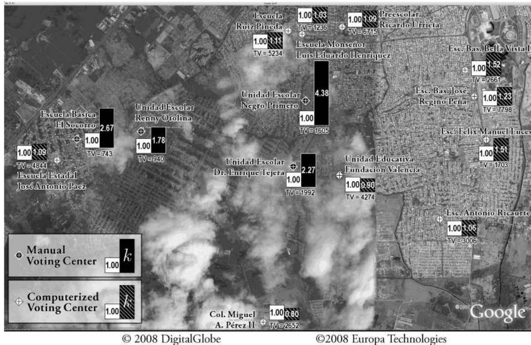
FIG. 16. Partial aerial view of Miguel Peña township (taken from the Google Earth™ mapping service). Manual versus computerized voting centers are compared in regards to their k value and total number of votes (TV). The image is centered at Latitude 10^{\circ}7'32.66''N and Longitude 68^{\circ}1'22.48''W .
