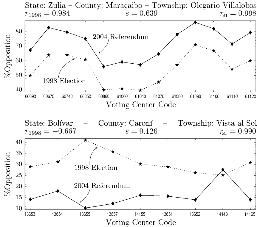
FIG. 9. Two sample townships. All the centers shown are computerized voting centers.
