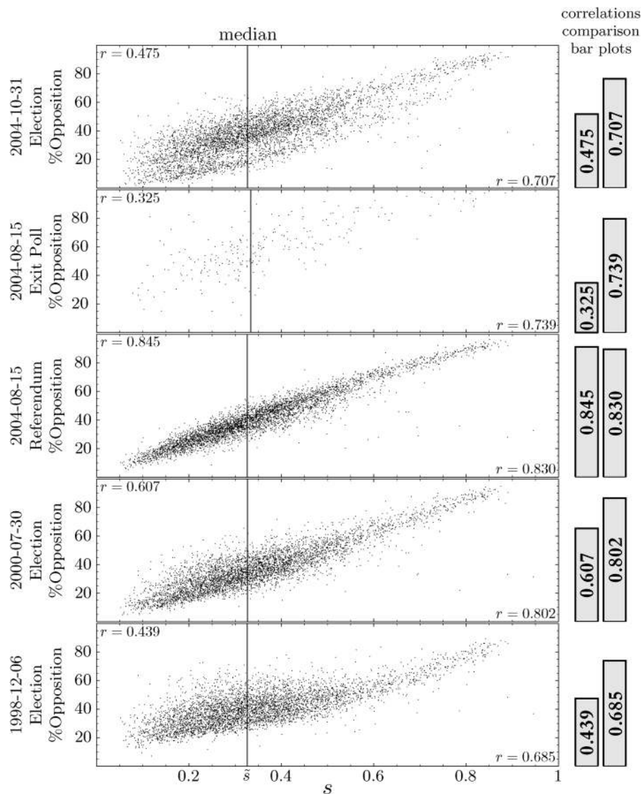
FIG. 11. Correlation between percentage of opposition and s for the lower two ( s \leq \tilde{s} ) and upper two quartiles ( s > \tilde{s} ) for computerized centers. The correlation for the lower two quartiles is expected to be smaller than the correlation in the upper two quartiles. This expected difference is not seen in the Referendum official results.
