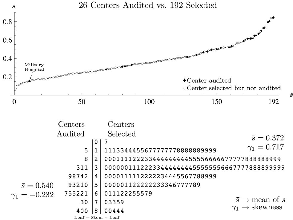
FIG. 13. Comparison between the s value of the 192 selected centers and the 26 audited centers. TOP: The selected centers are ordered according to the value of s and plotted. BOTTOM: Back-to-back stem-and-leaf plot showing the same values of s as in the top figure. To obtain s values, multiply stem by 0.1 and leaves by 0.01.
