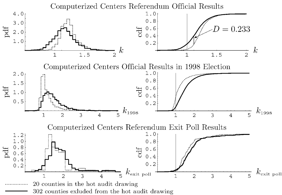
FIG. 23. Comparison of k probability density function (pdf) and cumulative density function (cdf) for computerized centers inside the 20 counties of the hot audit and in the 302 excluded counties. The maximum cdf difference (Supremum) for the official results is shown as D .
