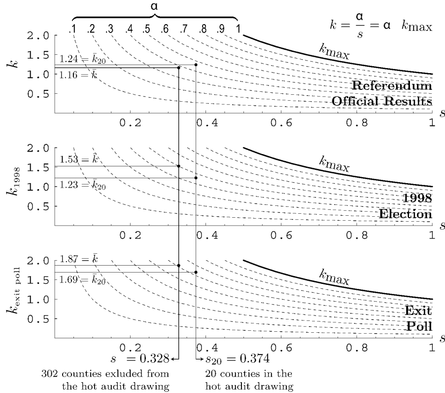
FIG. 22. Comparison of average k and s values for the computerized centers inside and outside the 20 counties to which the hot-audit universe was restricted. These \bar{k} and \bar{s} values are shown for the official referendum results, for the 1998 presidential election and for the referendum exit polls.
