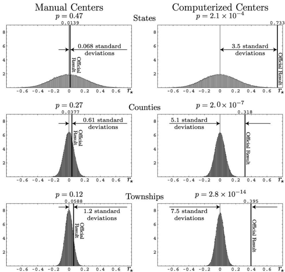
FIG. 20. Comparison of official results correlation r_* versus expected value distribution found after 100,000 simulations for manual and computerized centers at state, county or township level. The simulation results follow a normal distribution, which is shown as a dotted line. The probability of the official r_* happening by chance is indicated as p .
