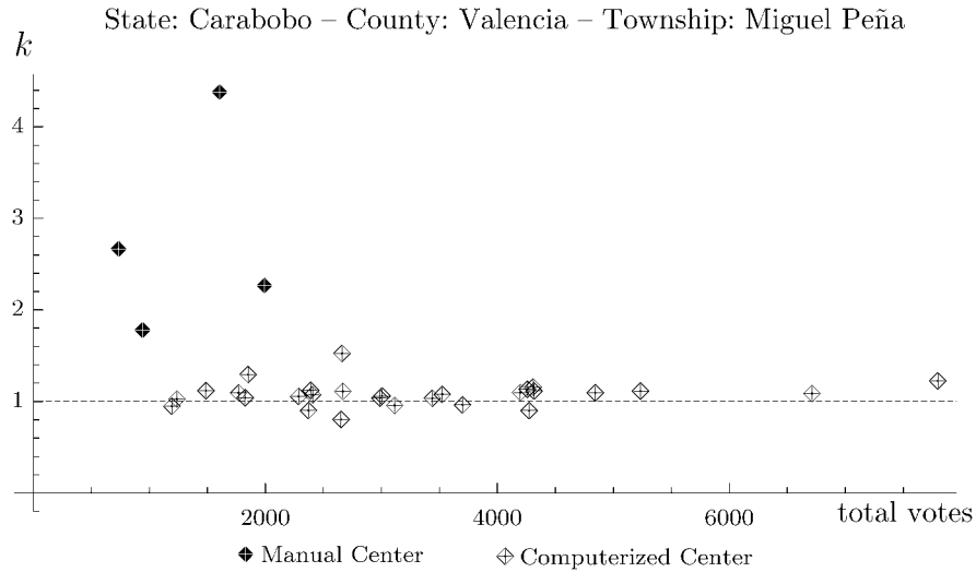
FIG. 17. Behavior of k versus total votes in all of Miguel Peña's voting centers. Manual and computerized centers are shown.
