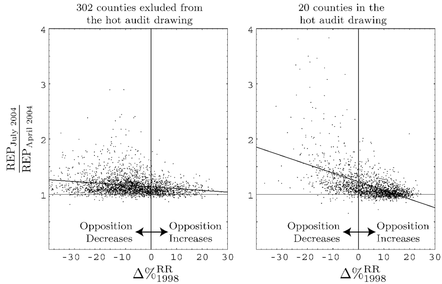
FIG. 24. REP variation versus \Delta\%RR_{1998} in computerized centers inside and outside the 20 counties of the hot-audit drawing. A least-square line is included in both cases.
