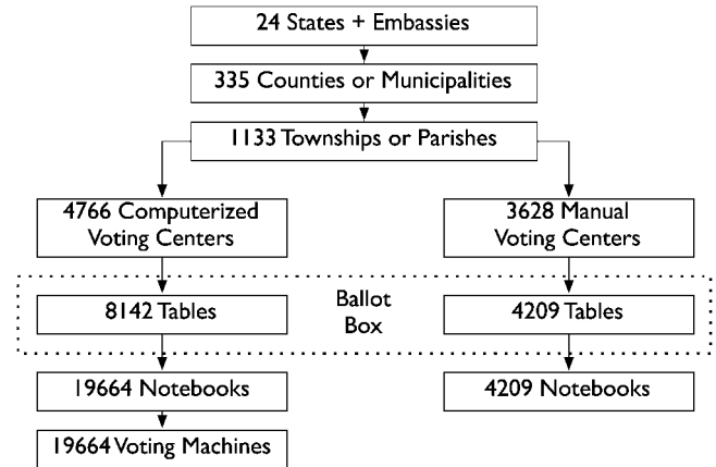
FIG. 1. Venezuelan vote collection structure.
