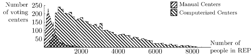
FIG. 2. Histogram of the size of the manual and the computerized centers.
