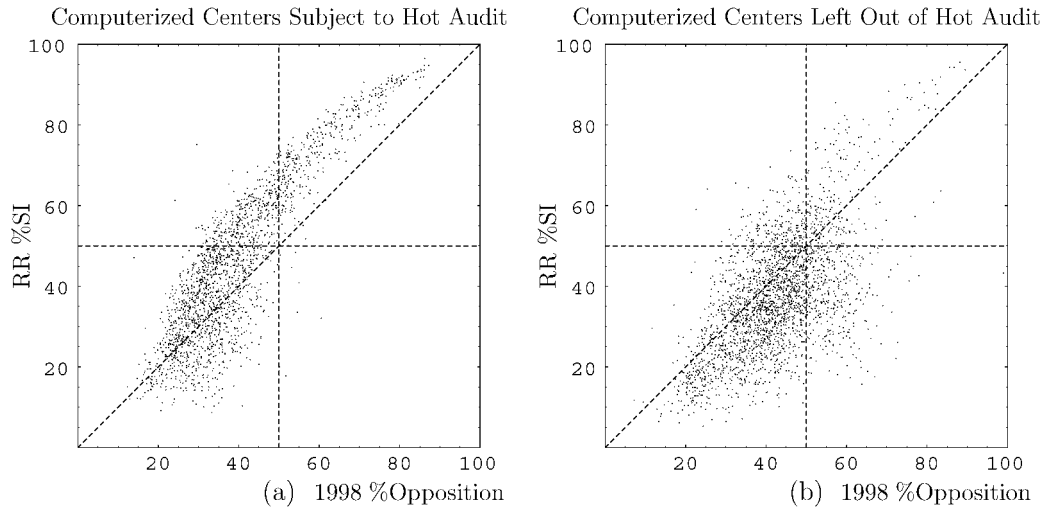
FIG. 12. Centers inside (a) and outside (b) of the 20 counties to where the hot-audit drawing was restricted.
