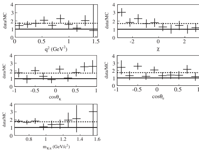
FIG. 7. Ratio (data/MC) distribution for Y(4S) decays versus each of the five kinematic variables. The dotted line corresponds to \text{data}/\text{MC} = 1.7 .
