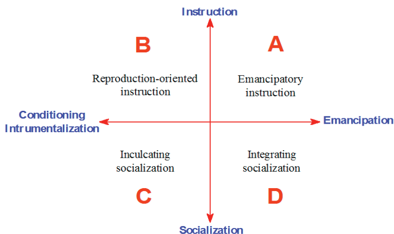
Figure 2. Tension between parameters associated with the conception of instruction and socialization (Lenoir, 2009).
