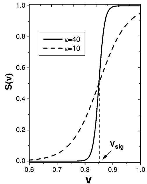
FIG. 4. Form of the function S(v) given by (9) for two values of the parameter \kappa .
