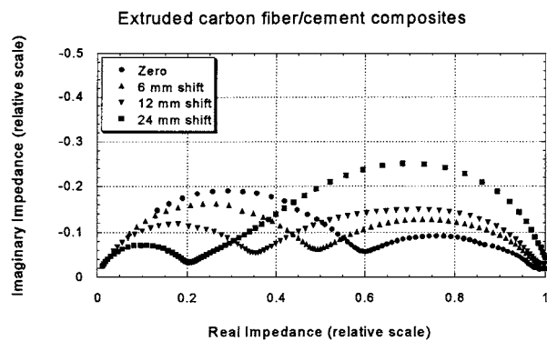
Figure 8 Experimental impedance spectra vs. orientation angle (shift of electrodes in Fig. 3c) for an extruded carbon fiber composite (0.5 vol% fibers). Electrode arcs are omitted and the data have been normalized by the DC resistance in each case—zero shift (1.9 k \Omega ), 6 mm shift (3.7 k \Omega ), 12 mm shift (8.2 k \Omega ), and 24 mm shift (27 k \Omega ).
