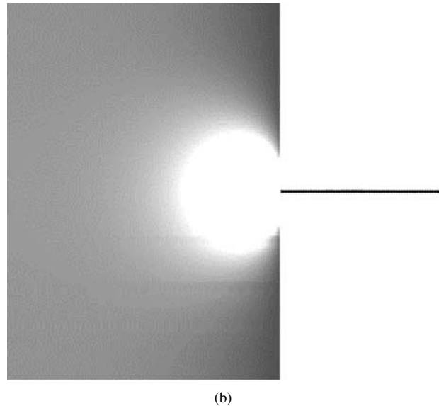
Figure 5 Showing (a) a schematic of the numerical cell used in the finite element simulation of the pull-out experiment, and (b) a gray scale image of the current density (current increases with lightness of gray scale) when the wire tip was just touching the water surface.
