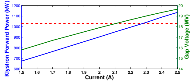
Figure 4: Optimal HER Gap Voltage and minimum necessary Klystron Forward Power versus Current.
