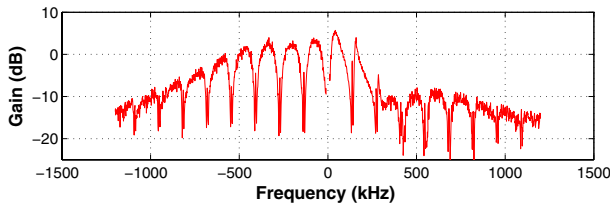
Figure 2: Frequency response distortion at high current.
