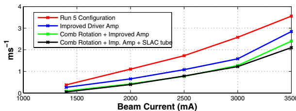
Figure 8: Estimated Growth Rates at 4.05\text{ MV} .
