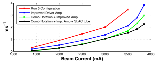
Figure 9: Estimated Growth Rates at 4.50\text{ MV} .
