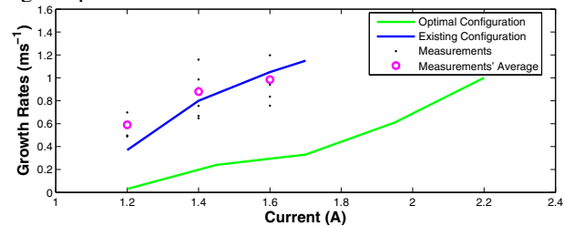
Figure 5: HER Growth Rates.
