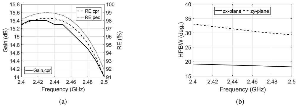
Fig. 7: Antenna radiation pattern simulation analysis versus frequency at 2.45 GHz. a Maximum simulated gain and RE for metallic parts considering as copper (cpr) and perfect electric conductor (pec). b HPBW in the zx - and zy - plane respectively.
