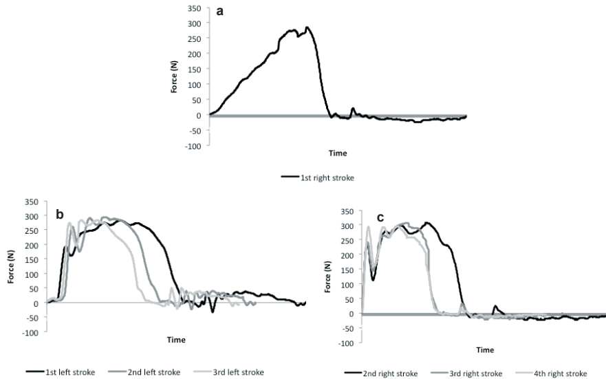
Figure 1: Force profile of the starting stroke (a) and three strokes in each side (left (b) and right (c)) by an elite female kayaker – SG-T.
