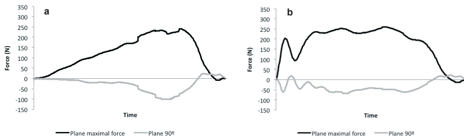
Figure 2: Force profile of two example strokes (on-water phases) with data from the SG-L and SG-T. Starting stroke (a) and a stroke performed with the kayak in movement (b).
