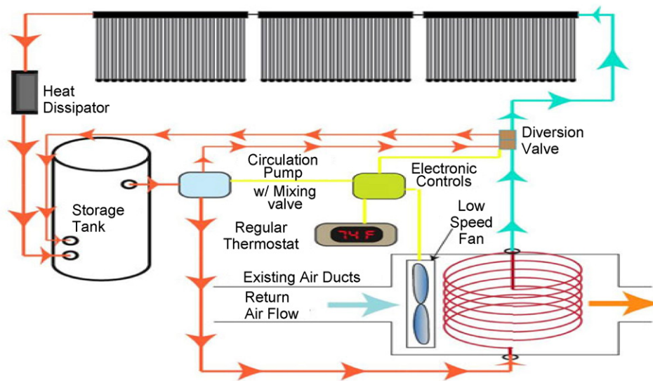
Fig. 2. Schematic diagram of the SWH system.
