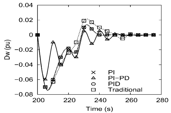
Figure 10. Comparison of the controllers when the system is submitted to a ramp \Delta P_6 = +0.23 pu .
