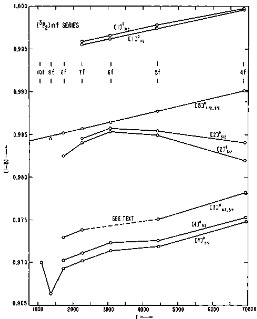
FIGURE 8. The (^3P_2)nf series plotted on a very expanded (1-5) scale to exhibit small perturbations.
