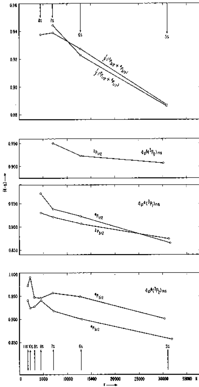
FIGURE 5. Diagram showing the observed Brt ns series.
