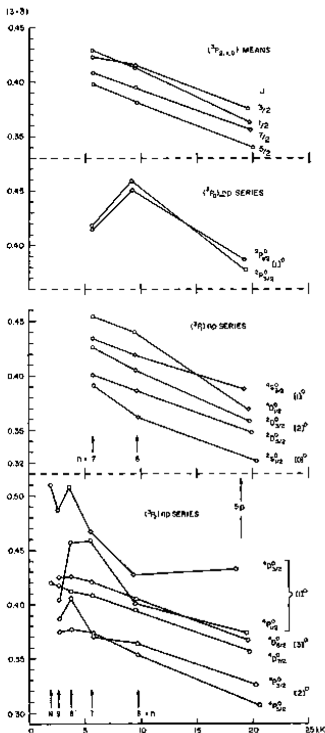
FIGURE 7. The (^3P_2)np series: (3-5) plotted against T .
