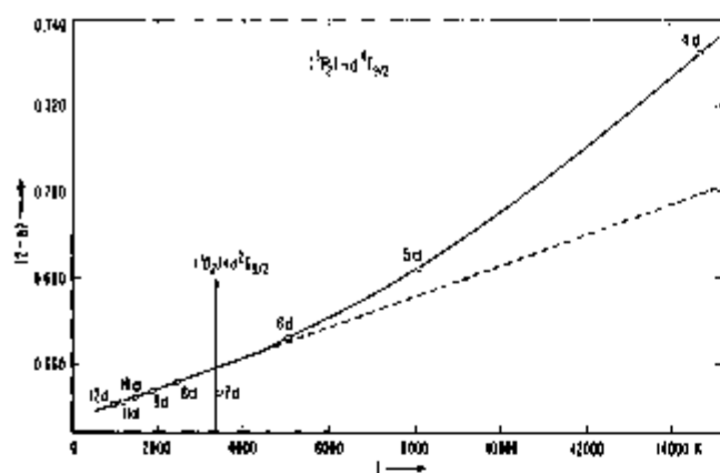
FIGURE 6. Diagram showing the very regular (^3P_2)nd\ ^4F_{3/2} series.
