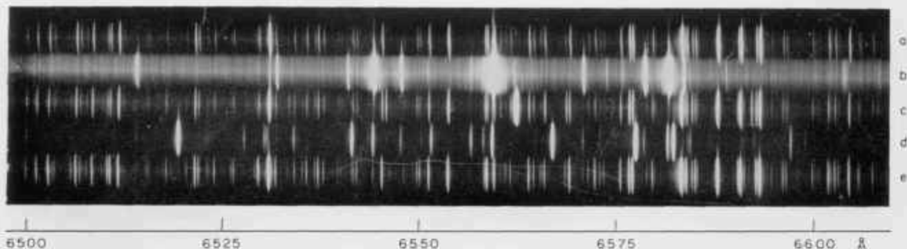
FIGURE 1. The bromine spectrum in the vicinity of H\alpha ( 6563 \text{ \AA} ).
