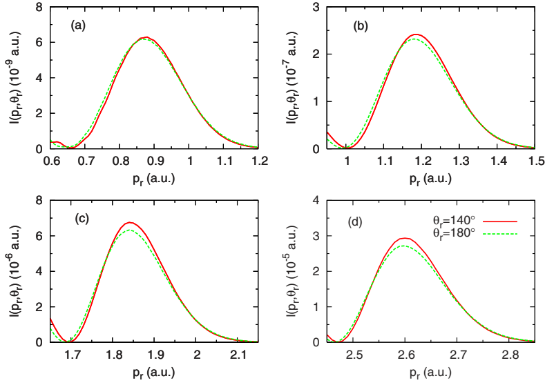
FIG. 8. (Color online) Distributions of the momentum of the right-side BRR electrons for atomic hydrogen by five-cycle laser pulses with the wavelength of 800 nm at the peak intensities of (a) 5.0 \times 10^{13} , (b) 1.0 \times 10^{14} , (c) 2.5 \times 10^{14} , and (d) 5.0 \times 10^{14} W/cm 2 .
