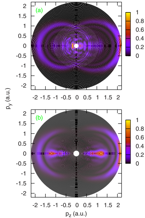
FIG. 2. (Color online) Photoelectron 2D momentum distributions parallel ( p_{\parallel}=p_z ) and perpendicular ( p_{\perp} ) to the laser polarization direction for atomic hydrogen by a five-cycle laser pulse with the wavelength of 800 nm at the peak intensity of 1.0 \times 10^{14} W/cm 2 . (a) SFA2 and (b) TDSE.
