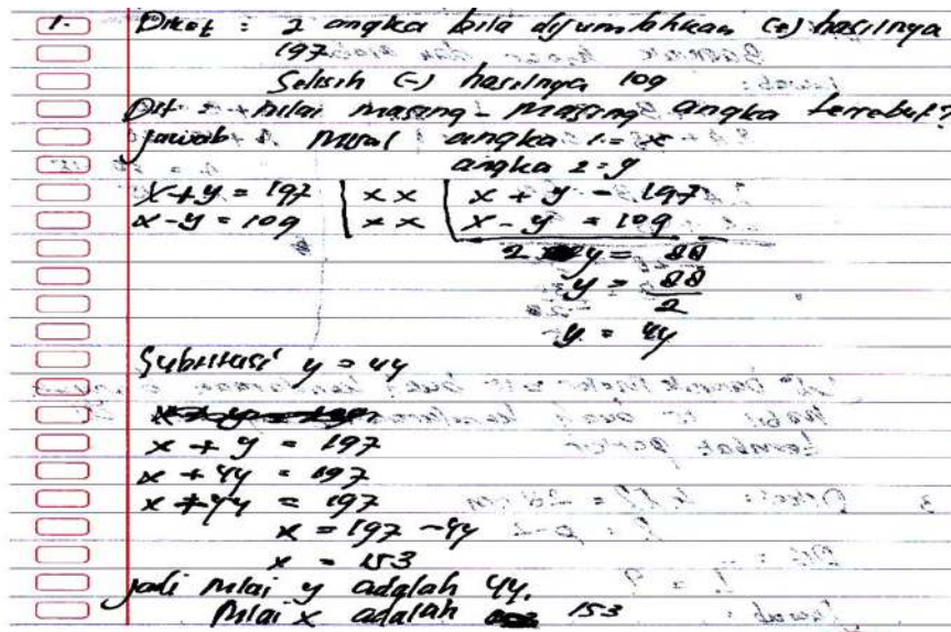
Figure 1. Student answers MF on question 1
