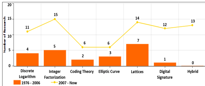
Figure 2. Number of research in PKC algorithm based on years
