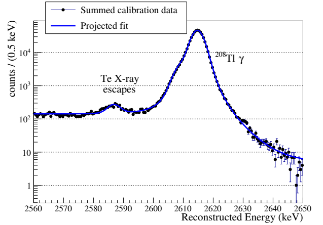
FIG. 8. Left : Best-fit model to the calibration 2615 keV peak for a single bolometer-dataset. The solid line shows the full summed model, and the dashed lines show the individual components: (a) the primary peak of the detector response; (b) the secondary peak of the detector response; (c) the smeared step-function; (d) the X-ray escape peak; (e) flat background. Right : The calibration spectrum summed over all BoDs pairs, with the summed best-fit model. Figure adapted from [11].
