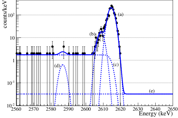
FIG. 8. Left : Best-fit model to the calibration 2615 keV peak for a single bolometer-dataset. The solid line shows the full summed model, and the dashed lines show the individual components: (a) the primary peak of the detector response; (b) the secondary peak of the detector response; (c) the smeared step-function; (d) the X-ray escape peak; (e) flat background. Right : The calibration spectrum summed over all BoDs pairs, with the summed best-fit model. Figure adapted from [11].
