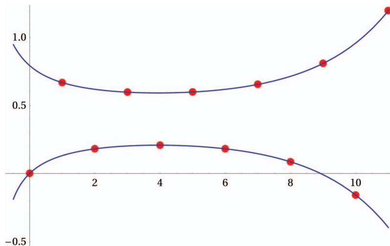
FIG. 1. S_{1,2,2}(-1, 2, -\frac{1}{3}; n) for n \in \{0, 1, \dots, 11\} , and f_e(\frac{n}{2}) , f_o(\frac{n-1}{2}) for n \in (-\frac{1}{2}, 11) .
