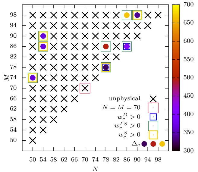
FIG. 3. (Color online) Illustration of configurations in (N, M) space with n_0 = 1 for the self-energy of a Sm atom, with relative noise of magnitude \sigma = 10^{-6} on Matsubara points. A black cross denotes an unphysical, \rho_c < 0 , continuation. A circular dot denotes a physical continuation, \rho_c \geq 0 , and the colour denotes the deviation \Delta_c .
