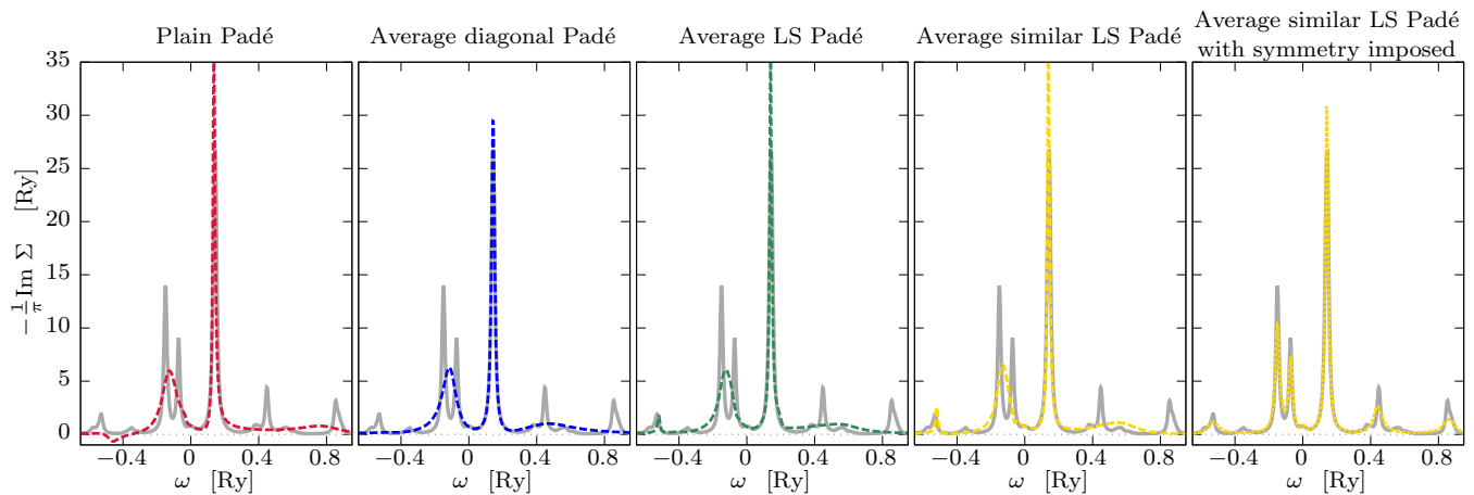
FIG. 2. (Color online) Illustration of the different improvements done on Plain Padé for a Sm atom, with relative noise of magnitude \sigma = 10^{-6} on the Matsubara points. Description of the five obtained spectra (from left to right panel): Plain Padé, using N = M = 70, n_0 = 1 , and characterised by unphysical features; Padé average with w_c^D and n_0 = 1 ; Padé average with w_c^{LS} and n_0 = 1 ; Padé average with w_c^S and n_0 = 1 ; Padé average with w_c^S and with mirror symmetry imposed by using n_0 \in \{-5:1:0\} .
