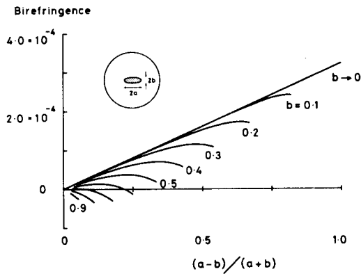
Fig. 5. Variation of modal birefringence with ellipticity in an elliptical core or jacket fiber plotted for various values of b , the ellipse minor axis.
