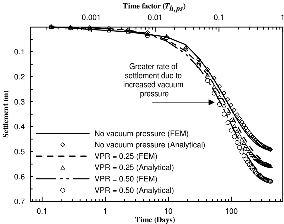
Figure 12. Settlement results from analytical and FEM solutions after conversion to equivalent plane strain condition, (a) Case A, short drain, (b) Case B, long drain.
