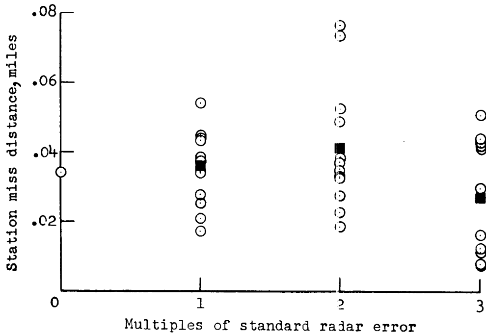
Figure 7.- Distribution and averaged values of the total velocity corrections and miss distances obtained during rendezvous as a function of the standard deviation of the radar errors.
