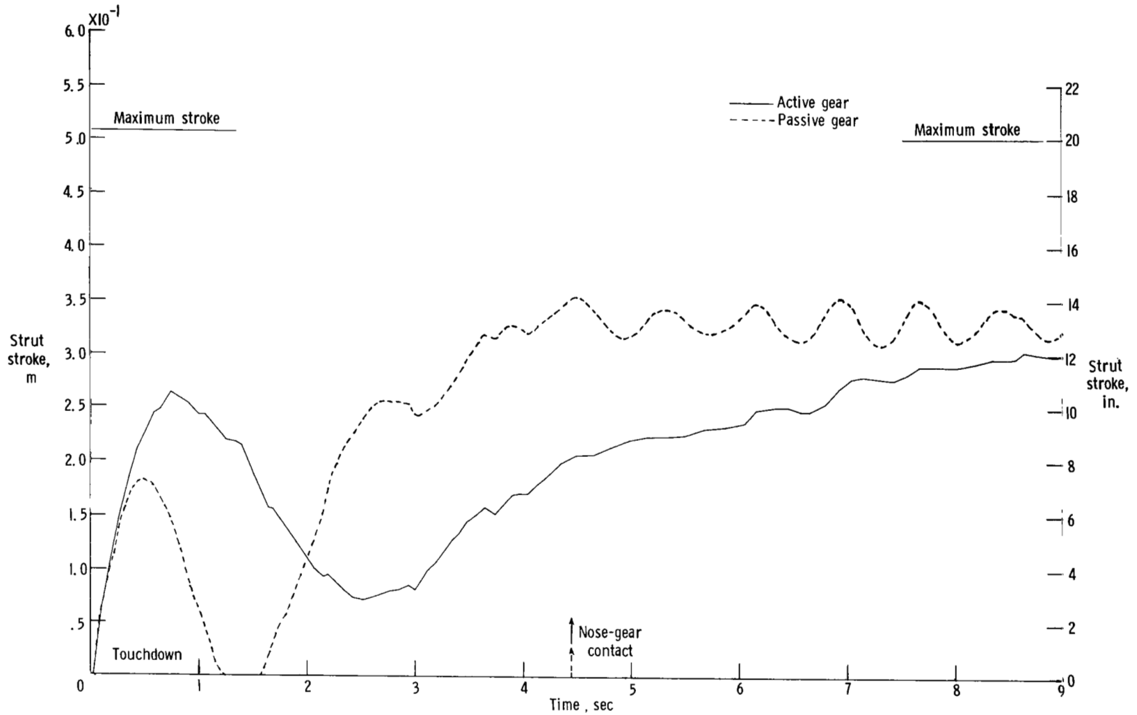
(1) Shock-strut strokes; large mass configuration; downhill runway.
