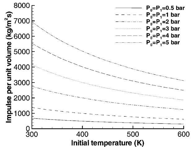
Fig. 26 Variation of impulse per unit volume with initial temperature for different values of the stagnation pressure.
