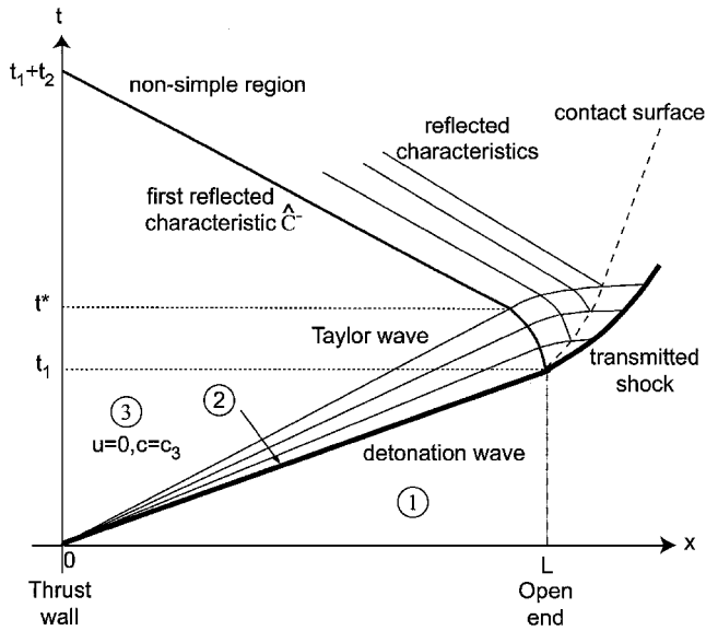
Fig. 4 Space-time diagram for detonation wave propagation and interaction with the tube's open end.
