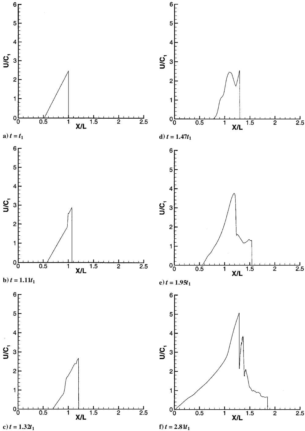
Fig. 7 Velocity along the tube centerline from numerical simulation; c_1 is the initial sound speed inside and outside the tube.
