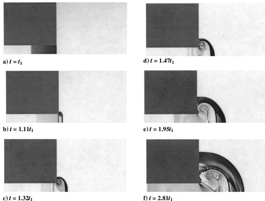
Fig. 5 Numerical schlieren images of the exhaust process.
