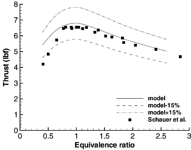
Fig. 15 Thrust prediction for a 50.8-mm diameter by 914.4 mm long hydrogen-air PDE operated at 16 Hz (comparison with experimental data of Schauer et al. 23 ); nominal initial conditions are P_1 = 1 bar and T_1 = 300 K, and lines corresponding to +15% and -15% deviation from the model values are also shown.
