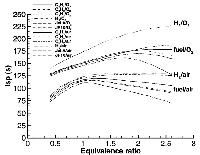
Fig. 21 Variation of mixture-based specific impulse with equivalence ratio; nominal initial conditions are P_1 = 1 bar and T_1 = 300 K.
