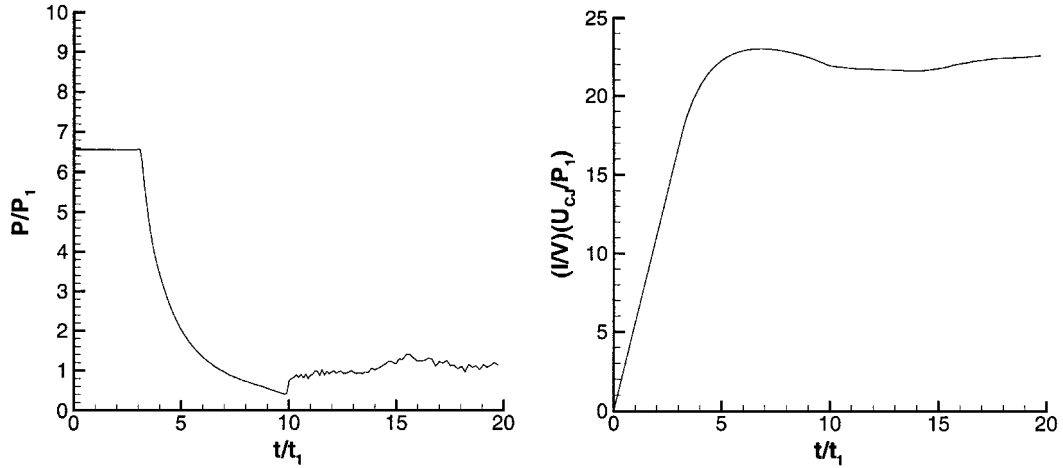
Fig. 8 Nondimensionalized thrust surface pressure and impulse per unit volume as a function of nondimensionalized time for the numerical simulation.
