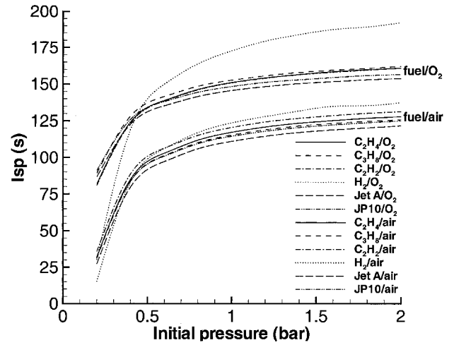
Fig. 20 Variation of mixture-based specific impulse with initial pressure; nominal initial conditions are T_1 = 300 K and stoichiometric fuel–oxygen ratio.
