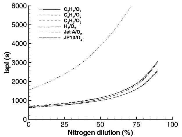
Fig. 25 Variation of fuel-based specific impulse with nitrogen dilution; nominal initial conditions are P_1 = 1 bar, T_1 = 300 K, and stoichiometric fuel–oxygen ratio.
