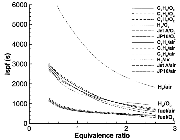
Fig. 24 Variation of fuel-based specific impulse with equivalence ratio; nominal initial conditions are P_1 = 1 bar and T_1 = 300 K.
