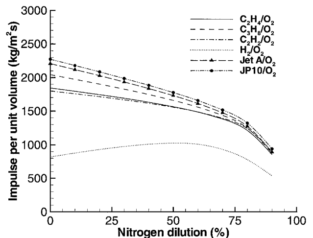
Fig. 19 Variation of impulse per unit volume with nitrogen dilution; nominal initial conditions are P_1 = 1 bar, T_1 = 300 K, and stoichiometric fuel-oxygen ratio.
