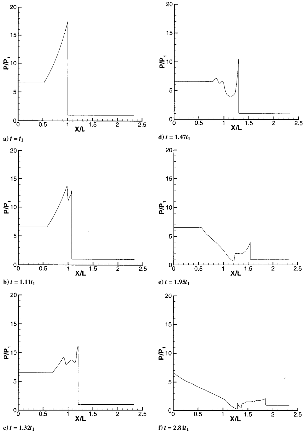
Fig. 6 Pressure along the tube centerline from numerical simulation; P_1 is the initial pressure inside and outside the tube.
