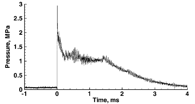
Fig. 10 Sample pressure recorded at the thrust surface 9 for a mixture of stoichiometric ethylene–oxygen at 1-bar and 300-K initial conditions.
