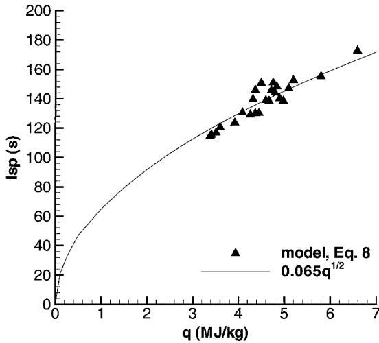
Fig. 16 Specific impulse scaling with energy content; model predictions [Eq. (8)] vs effective specific energy content q for hydrogen, acetylene, ethylene, propane, and JP10 with air and oxygen including 0, 20, 40, and 60% nitrogen dilution at P_1 = 1 bar and T_1 = 300 K.
