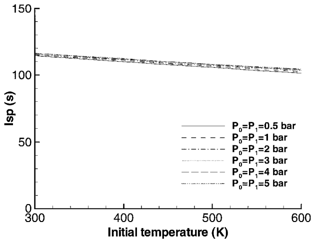
Fig. 27 Variation of mixture-based specific impulse with initial temperature for different values of the stagnation pressure.
