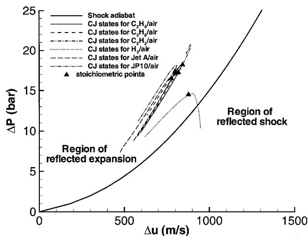
Fig. 3 Pressure–velocity diagram used to compute wave interactions at the tube open end for fuel–air mixtures.
