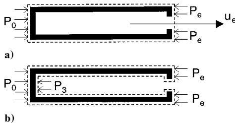
Fig. 9 Control volumes a) typically used in rocket engine analysis and b) used in our analysis.
