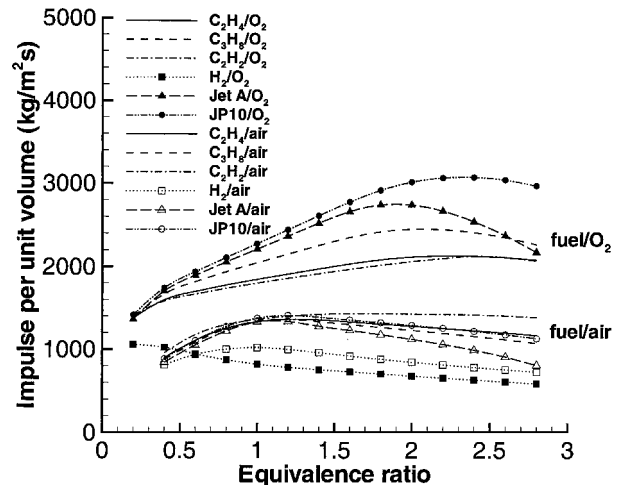
Fig. 18 Variation of impulse per unit volume with equivalence ratio; nominal initial conditions are P_1 = 1 bar and T_1 = 300 K.
