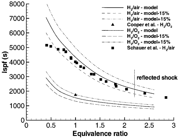
Fig. 13 Comparison of specific impulse between model predictions and experimental data for hydrogen-air 23 with varying equivalence ratio and stoichiometric hydrogen-oxygen 9 ; nominal initial conditions are P_1 = 1 bar and T_1 = 300 K, and lines corresponding to +15% and -15% deviation from the model values are also shown.
