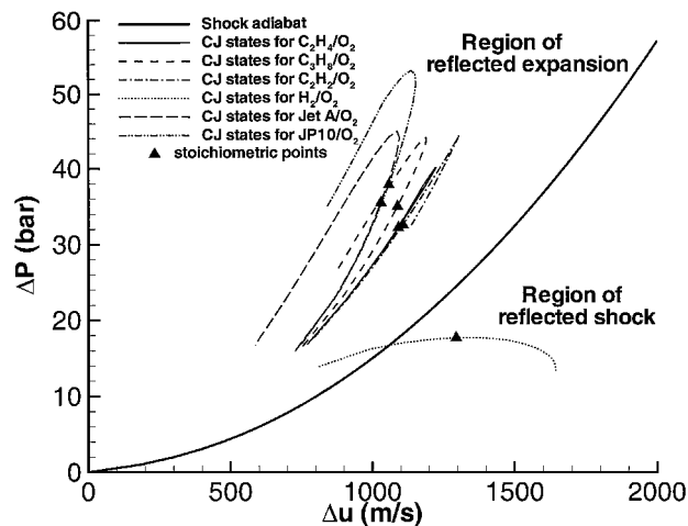
Fig. 2 Pressure–velocity diagram used to compute wave interactions at the tube open end for fuel–oxygen mixtures.
