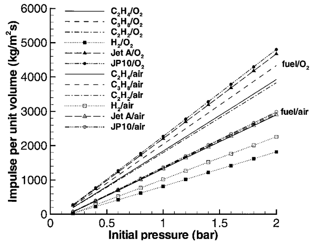
Fig. 17 Variation of impulse per unit volume with initial pressure; nominal initial conditions are T_1 = 300 K, stoichiometric fuel-oxygen ratio.
