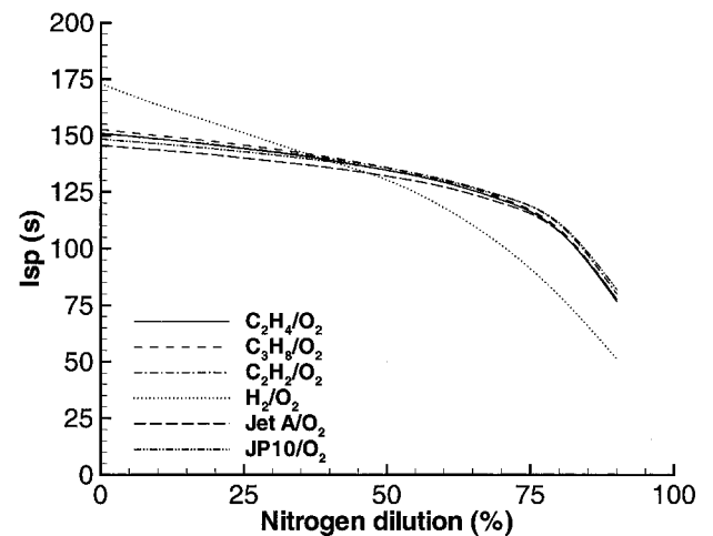
Fig. 22 Variation of mixture-based specific impulse with nitrogen dilution; nominal initial conditions are P_1 = 1 bar, T_1 = 300 K, and stoichiometric fuel–oxygen ratio.
