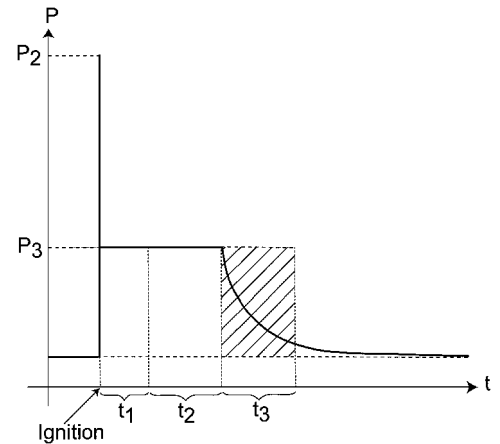
Fig. 11 Idealized model of the thrust surface pressure history.
