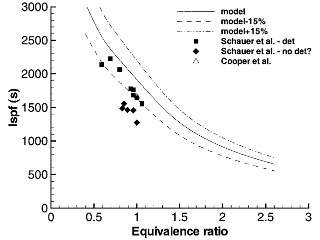
Fig. 14 Comparison of specific impulse between model predictions and experimental data 9,24 for propane-air with varying equivalence ratio; nominal initial conditions are P_1 = 1 bar and T_1 = 300 K, and lines corresponding to +15% and -15% deviation from the model values are also shown.
