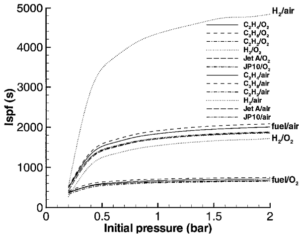
Fig. 23 Variation of fuel-based specific impulse with initial pressure; nominal initial conditions are T_1 = 300 K and stoichiometric fuel–oxygen ratio.
