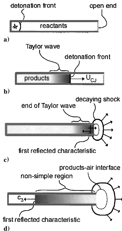
Fig. 1 Pulse detonation engine cycle: a) detonation is initiated at the thrust surface; b) detonation, followed by the Taylor wave, propagates to the open end of the tube at a velocity U_{CJ} ; c) expansion wave is reflected at the mixture-air interface and immediately interacts with the Taylor wave while the products start to exhaust from the tube; and d) first characteristic of the reflected expansion reaches the thrust surface and decreases the pressure at the thrust surface.
