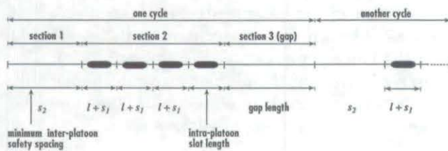
Fig. 12. Platoon/gap cycle.
