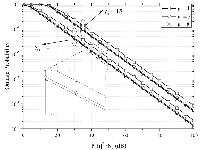
FIGURE 7. Outage probability vs \frac{P||h_l|^2}{N_o} for different values of \mu and \gamma_{th} , assuming ideal RF front-end and d = 30 m.
