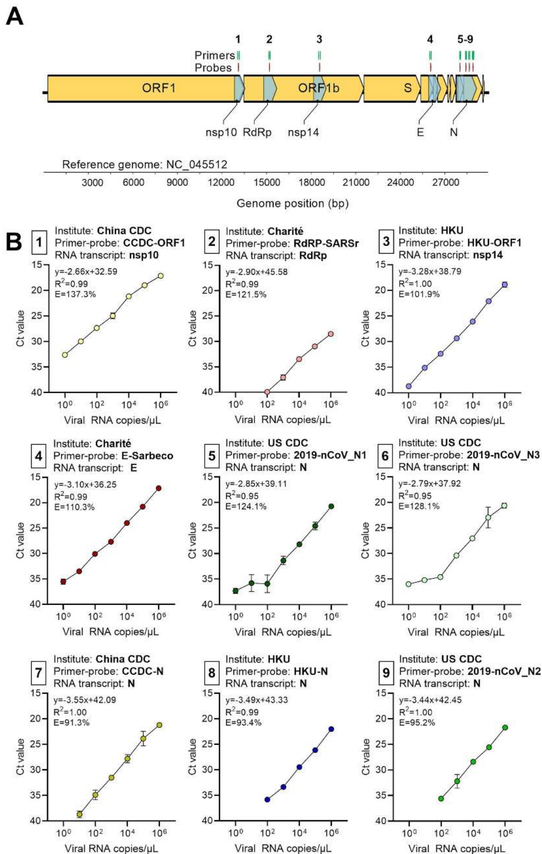
Fig. 1: Generation of RNA transcript standards for validation of SARS-CoV-2 qRT-PCR assays. (A) We reverse-transcribed RNA transcript standards for the non-structural protein 10 (nsp10), RNA-
