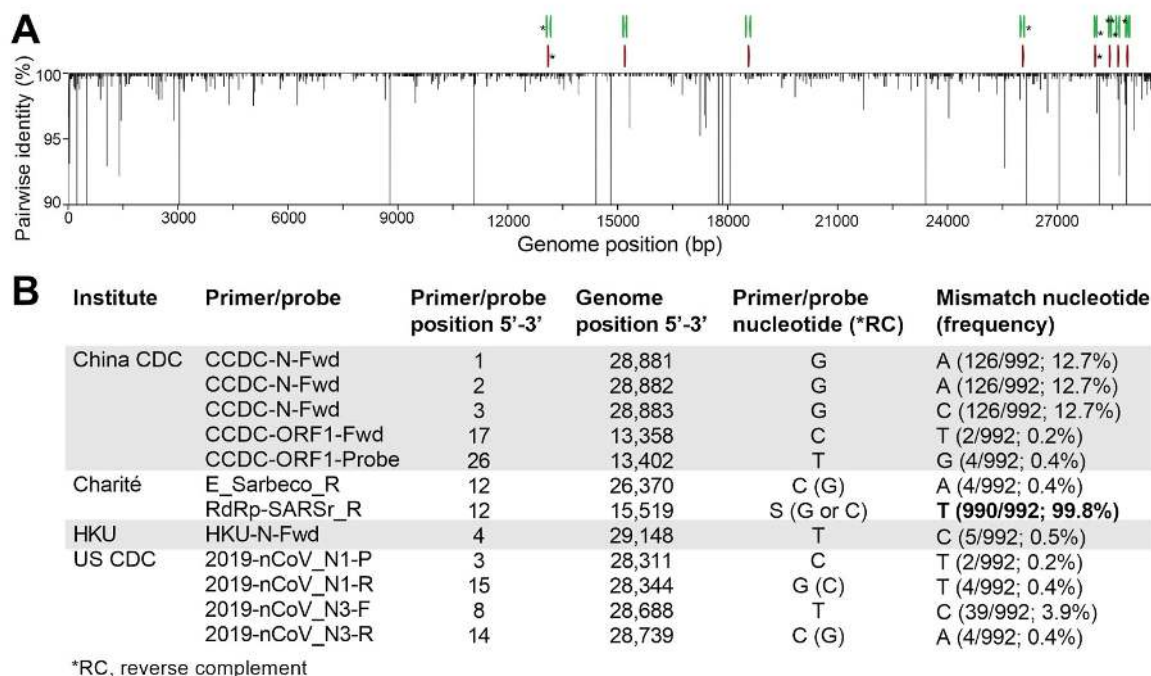
Fig. 6: High frequency primer and probe mismatches may result in decreased sensitivity for SARS-CoV-2 detection. (A) We aligned nucleotide diversity across 992 SARS-CoV-2 genomes sequenced up to 22 March 2020 and determined mismatches with the nine primer-probe sets. We measured diversity using pairwise identity (%) at each position, disregarding gaps and ambiguous nucleotides. Asterisks (*) at the top indicate primers and probes targeting regions with one or more mismatches. Genomic plots were designed using DNA Features Viewer in Python 16 . (B) We only listed mismatch nucleotides with frequencies above 0.1%. These mismatches may result in decreased sensitivity of primer-probe sets.
