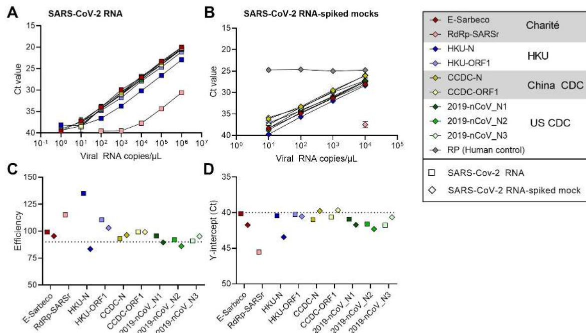
Fig. 2: Analytical efficiency and sensitivity of the nine primer-probe sets used in SARS-CoV-2 qRT-PCR assays. We compared nine primer-probe sets and a human control primer-probe set targeting the human RNase P gene with 10-fold dilutions of (A) full-length SARS-CoV-2 RNA and (B) pre-COVID-19 mock samples spiked with known concentrations of SARS-CoV-2 RNA. We determined (C) efficiency and (D) y-intercept Ct values (measured analytical sensitivity) of the nine primer-probe sets. We extracted nucleic acid from SARS-CoV-2-negative nasopharyngeal swabs (collected from respiratory disease patients in 2017) and spiked these with known concentrations of SARS-CoV-2 RNA. Symbols depict sample types: squares represent tests with SARS-CoV-2 RNA and diamonds represent
